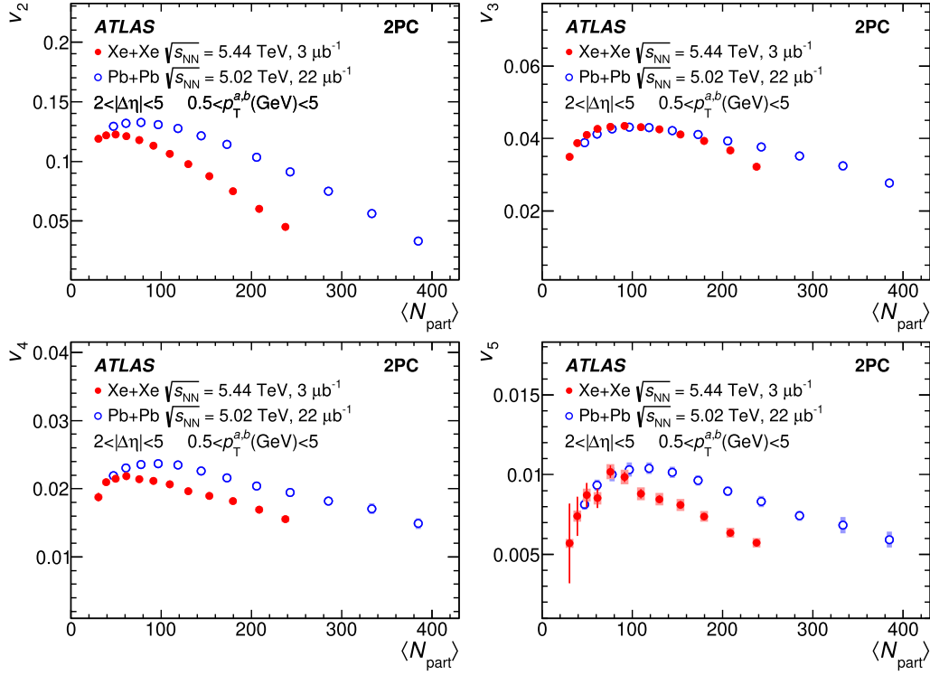
FIG. 18. Comparisons of the v_n as a function of \langle N_{\text{part}} \rangle measured in Xe + Xe collisions with those measured in Pb + Pb collisions at \sqrt{s_{NN}} = 5.02 TeV. Each panel corresponds to a different harmonic order n . The plots are for the 2PC method and for 0.5 < p_T^b < 5 GeV. The error bars and bands represent statistical and systematic uncertainties, respectively.
