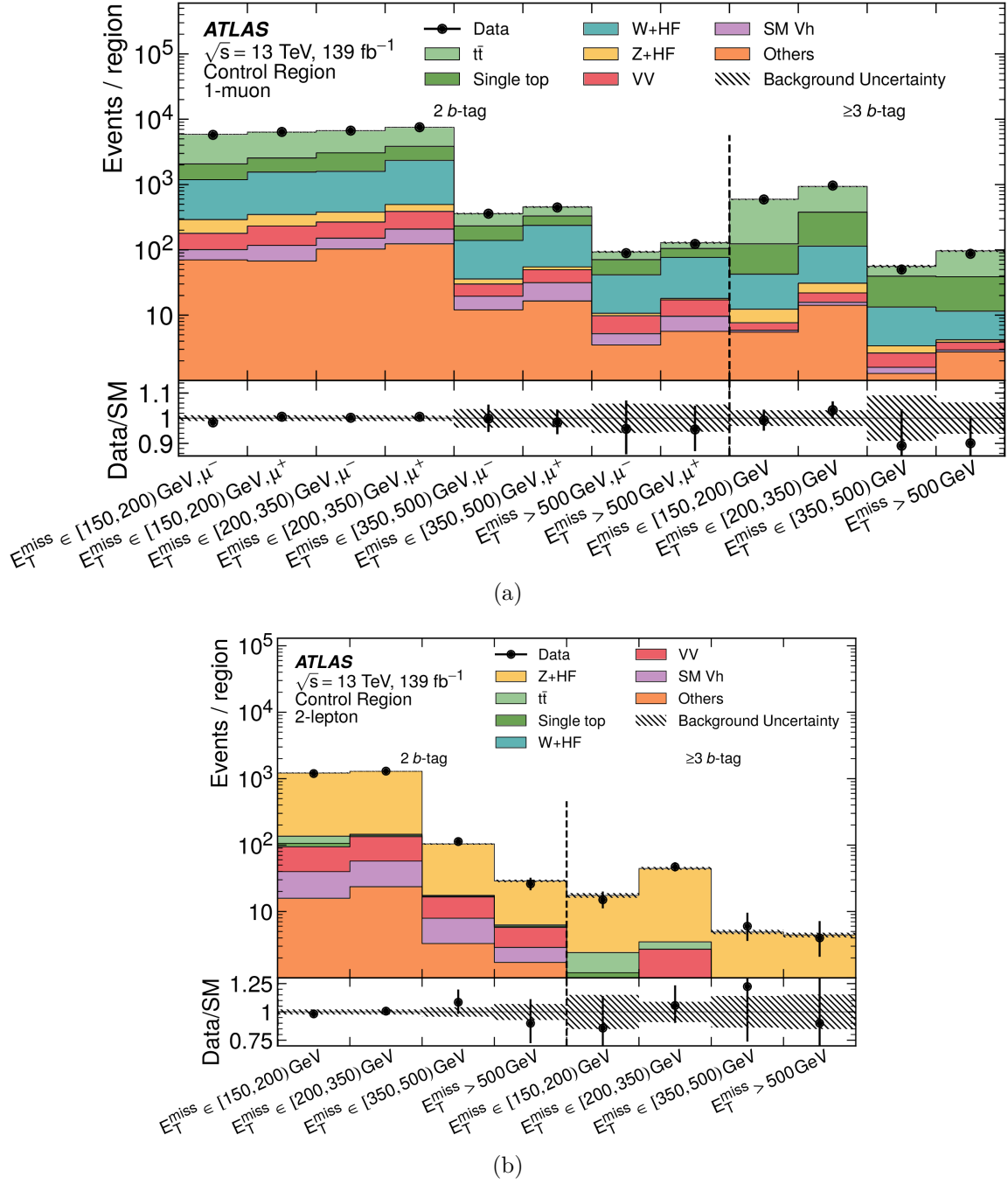
Figure 3. Yields in the resolved and merged (a) 1-muon control regions and (b) 2-lepton control regions. The top panel compares the fitted background yields with data, while the bottom panel indicates the ratio of the observed data to the predicted Standard Model backgrounds. The different control region bins included in the fit are indicated on the x -axis by first giving the range in E_T^{\text{miss}} and then the sign of the muon charge (where applicable).
