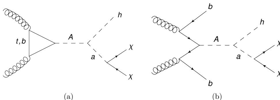
Figure 2. Feynman diagrams for the main production mechanisms of the mono-Higgs signature in the 2HDM+ a scenario: (a) gluon-gluon fusion and (b) b -associated production.
