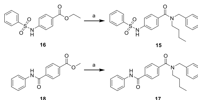
Scheme 2. Synthesis of Reverse Sulfonamide 15 and Amide Analogue 17 a
