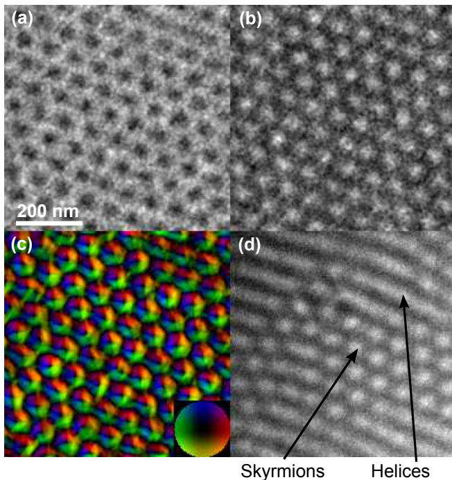
FIG. 1: (a),(b) Skyrmions in \text{Cu}_2\text{OSeO}_3 imaged with Lorentz TEM at 10 K in a field of 30 mT with defoci \pm 0.7 \mu\text{m} . (c) Magnetic induction map constructed from (a) and (b) using the transport of intensity equation. The direction of the local induction is indicated by the colour wheel (inset). (d) Skyrmions coexisting with the helical phase at 30 K in a field of 40 mT. Similar observations were made by Seki et al. 8
