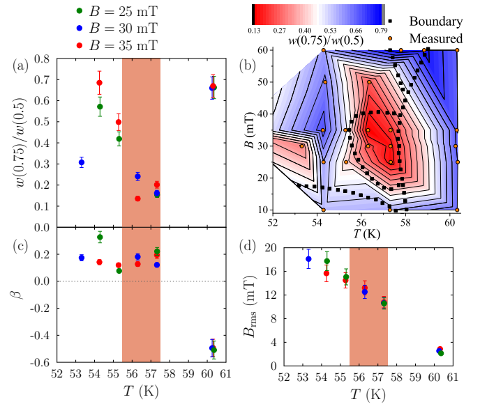
FIG. 5: (a) The ratio of peak widths w(0.75)/w(0.5) discussed in the text. (b) Contour plot of w(0.75)/w(0.5) from which the SkX phase may be identified. (c) The skewness \beta and (d) standard deviation B_{\text{rms}} as a function of temperature.
