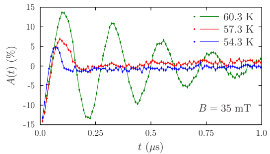
FIG. 3: (a) Time domain spectra measured in an applied transverse magnetic field of 35 mT in the paramagnetic phase at 60.3 K, the skyrmion phase at 57.3 K and the single- q phase at 54.3 K.
