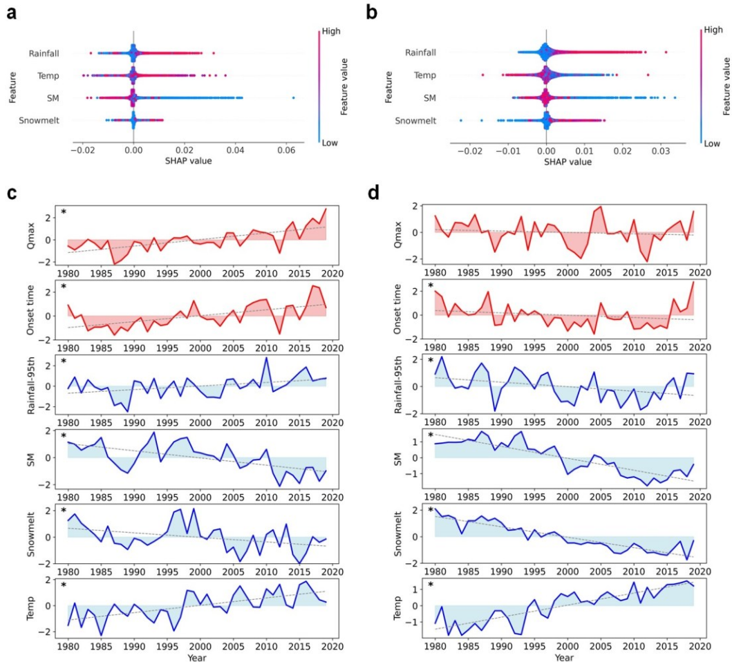
Figure 8. Attribution of flashier floods in Q-dominated and T-dominated basins. Two basin types
