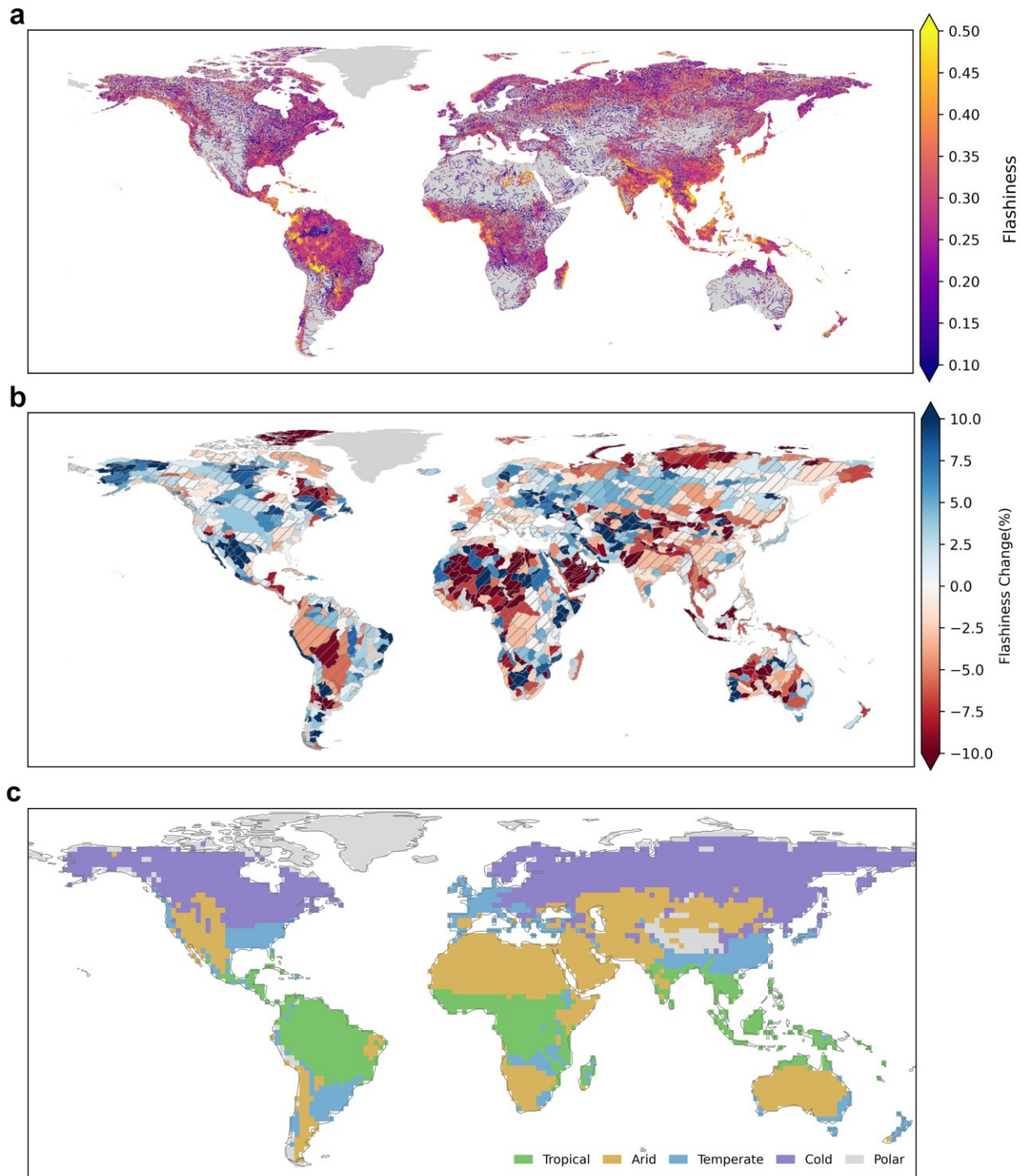
Figure 2. Global patterns of river reach-based flashiness, its temporal changes, and climatic context. (a) Present-day flashiness indices calculated for the period 1980 to 2019. (b) Percent change from the early period (1980–1999) to the later period (2000–2019) in the flashiness indices
