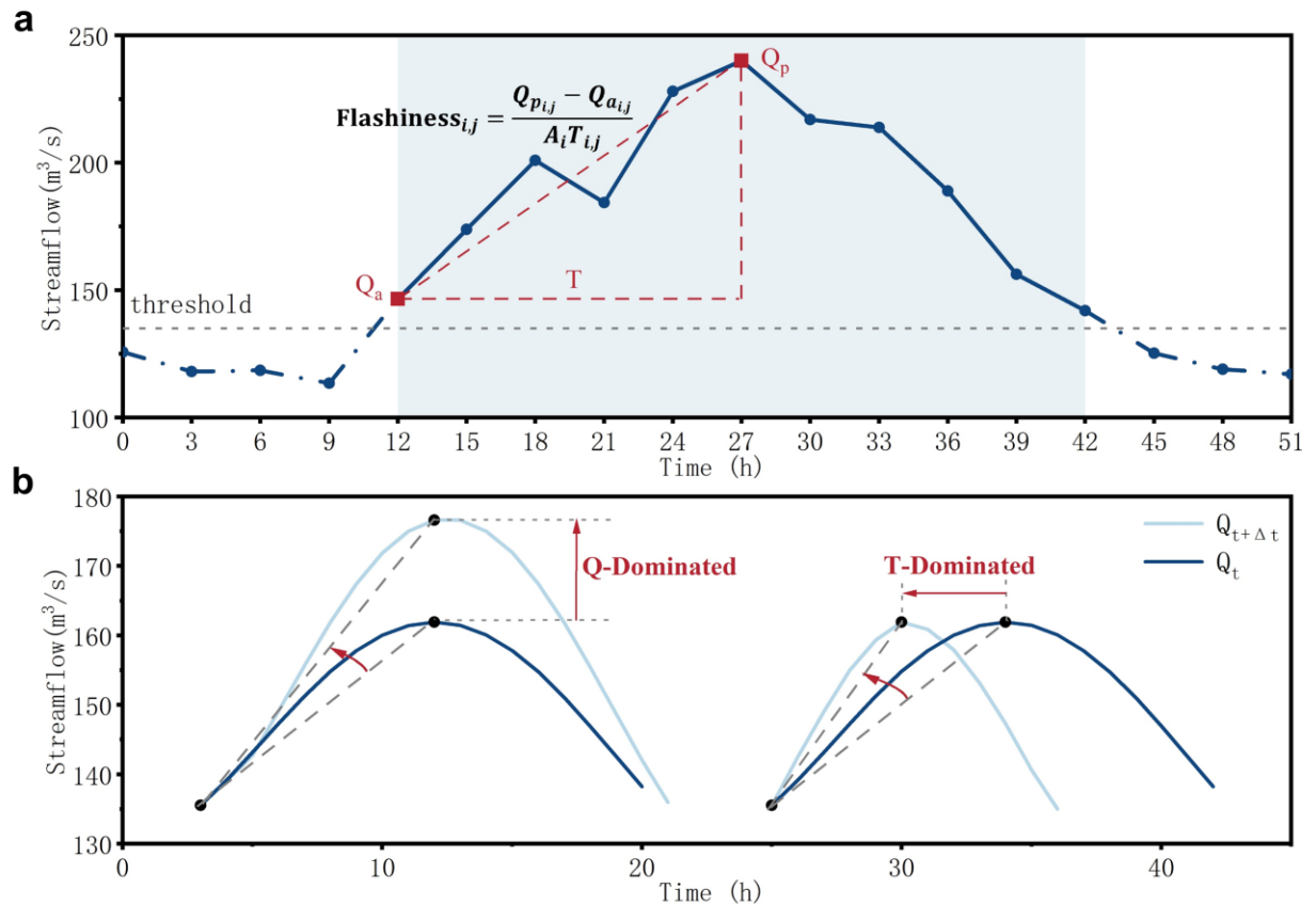
Figure 1. Definition of flashiness and classification of increasing flashiness. (a) Schematic
