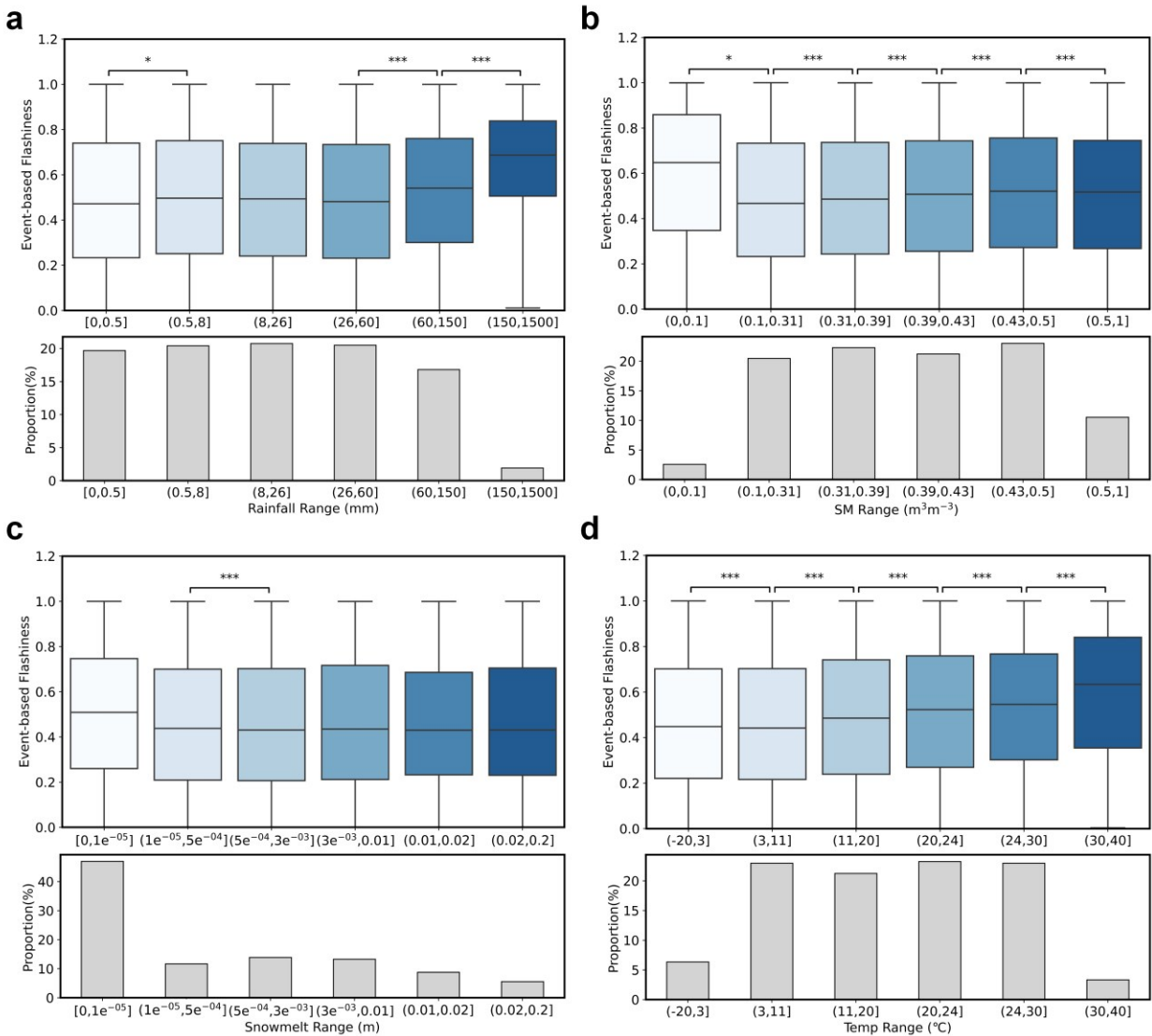
Figure 3. Relationship between event-based flashiness and different factors. The upper panels (a-d) display boxplots of flashiness statistics across varying ranges of key factors: (a) rainfall, (b) soil
