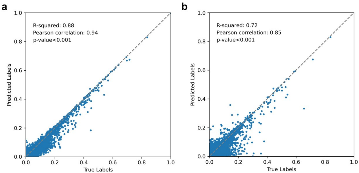
Figure 7. Model performance of LightGBM. (a-b) Scatter density plots of observations and predictions of the LightGBM model for the training (a) and test (b) datasets.
