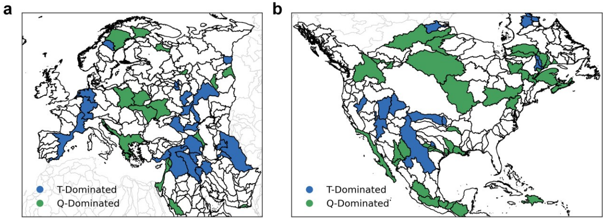
Figure 6. Classification of Level 4 basins with significant increases in flashiness. (a) Classification of basins exhibiting significant increases in flashiness across Europe. The blue regions represent areas in which the increase in flashiness is predominantly influenced by a shortened onset time, whereas the green regions represent areas where the increase in flashiness is primarily influenced by higher flood peak discharge. (b) Similar to a, but for basins across North America.
