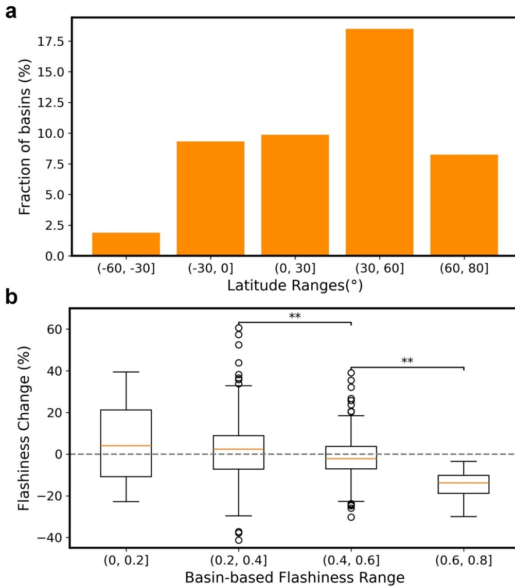
Figure 4. Statistical distribution of flashiness changes in global basins. (a) Statistics on the fraction
