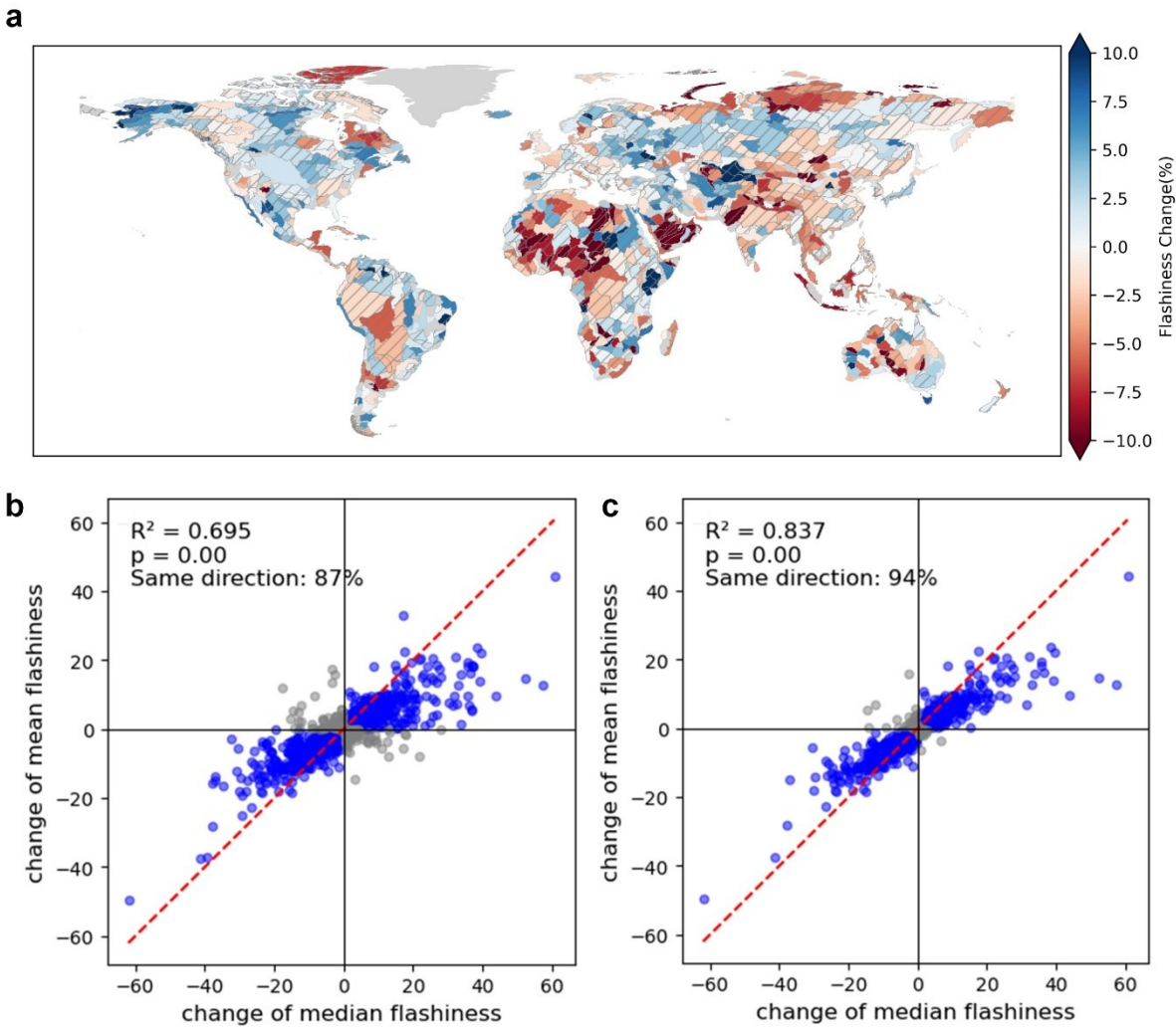
Figure 5. Comparison of flashiness changes aggregated using mean empirical cumulative distribution function (ECDF) versus median ECDF. (a) Similar to Figure 1b in the main text, but
