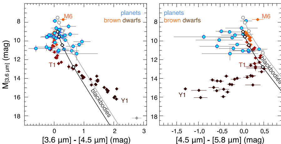
Fig. 22 Mid-infrared colour-magnitude diagrams, using Spitzer's IRAC photometric system. The daytime emission of transiting exoplanets are represented as blue dots, while the coloured diamonds show ultra-cool dwarfs from spectral type M6 to Y1. The two lines show the locus of blackbodies with 1 R_{\text{jup}} (black) and 2 R_{\text{jup}} (grey). Planets do not follow this: they are not blackbodies. The systematic bias from the blackbody, on the right panel, indicates the presence of water in the population of planets. Whereas individual measurements were unable to extract this information, taken as a group, there is a significant detection. Adapted from [230]
