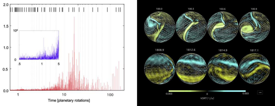
Fig. 30 Left: Power spectrum of the quasi-periodic disk-integrated radiation flux centred on east terminator time series; the high-frequency part of the spectrum is shown in the inset. Strong peaks are demarcated at the top. The strongest peaks are in the 10–20 day periods, with the strongest at ~17 day period, in this case. Right: Multiple equilibria of hot-Jupiter atmospheres: two circulation states are exhibited from a single simulation. The top row shows a state characterized by cyclogenesis (formation of cyclonic storms), alternating in the northern and southern hemispheres. The Bottom row shows a state characterized by a translating dipole-pair, which is nearly phase-locked. Transitions between the two states, as well as a small number of others, are seen in long-duration simulations (fig. Credit, James Cho)
