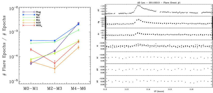
Fig. 49 Left: Probability ( \# \text{ Flare Epochs} / \# \text{ Epochs} ) to detect a flare for stars from M0 to M6 as a function of the band. Right: Multi-wavelength observations of a bright flare in AD Leo. The entire time span is 30 min. The variation in the U band is of the order of 1.5 magnitude (at peak) while the upper limit in K is less than 0.02 mag
