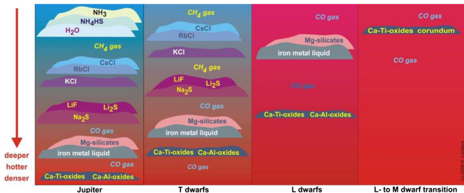
Fig. 5 Cloud layers in atmospheres ranging from our Jupiter to the hottest brown dwarfs (figure from [142]). Condensate clouds of various species form at specific points in the temperature - pressure profile. As atmospheres cool, these clouds sink deeper, falling below the observable gaseous layer
