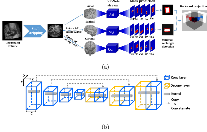
Figure 2: Networks design details: (a) An overview of the CNN-based image analysis pipeline. A raw ultrasound volume is preprocessed using our skull-stripping tool. The masked brain image and two of its transformed ( 90^\circ rotation) volume are passed, in parallel, to three independent VP-Nets. Each VP-Net outputs the projection mask of five structures (15 projected masks for 5 structures). The minimal rectangle that encloses the prediction silhouette is detected for each structure in each view, to generate the bounding box parameters. The 3D bounding box for a structure can be reconstructed with two obtained rectangle masks with backward projection. A graphical demo for the VP-Net model is available at: https://youtu.be/KVxkbqWYWxc . (b) Each individual VP-Net shares the same spirit as 2D U-Net [25] for full-resolution prediction. In VP-Net, convolution filters in all layers only scan along the 2D X-Y plane, while always penetrating along the Z-axis to capture contextual information along that dimension.
