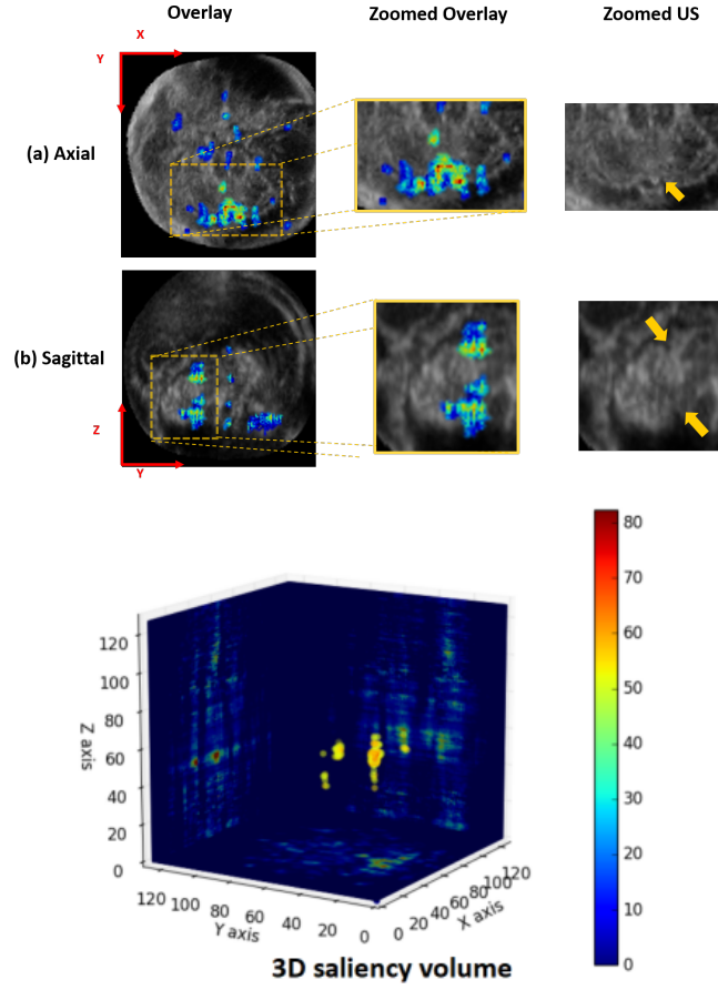
Figure 8: Visualization of a 3D saliency volume derived from CE detection in the axial view. The right-hand figure shows the points with top 2% gradient values in 3D. The color red represents higher gradient values, indicating a higher influence on the prediction outcome. Sub-figure (a)(b) shows a axial and a sagittal US slice with 3D saliency points projected on each view respectively. The images and the original US are zoomed in for detail visualization.
