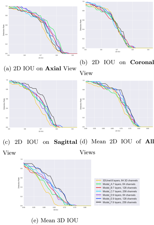
Figure 7: Mean 2D & 3D IOU curves of 3D U-Nets (yellow) and VP-Nets (other colors). b.shows 3D U-Nets perform similarly with other VP-Nets on coronal view in 2D IOU. All VP-Nets achieves higher accuracy when combine the three views together (e). Comparing different variants of VP-Nets, Model F(black) achieves the highest accuracy. It shows that larger feature channel and deeper layers increase the network performance.
