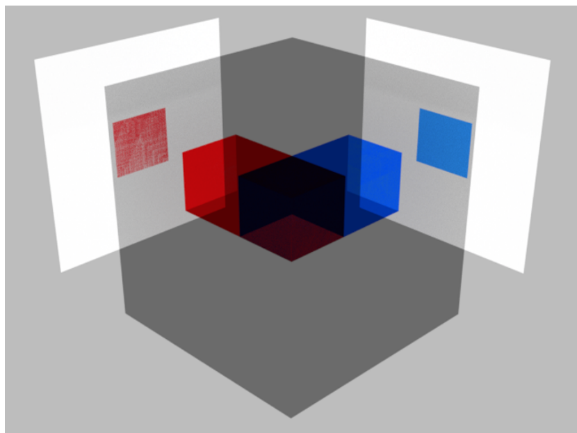
Figure 5: Back-ward projection. The red and blue are rectangle masks detected from two different views. The 3D bounding box can be obtained by intersection of their projection (dark purple).
