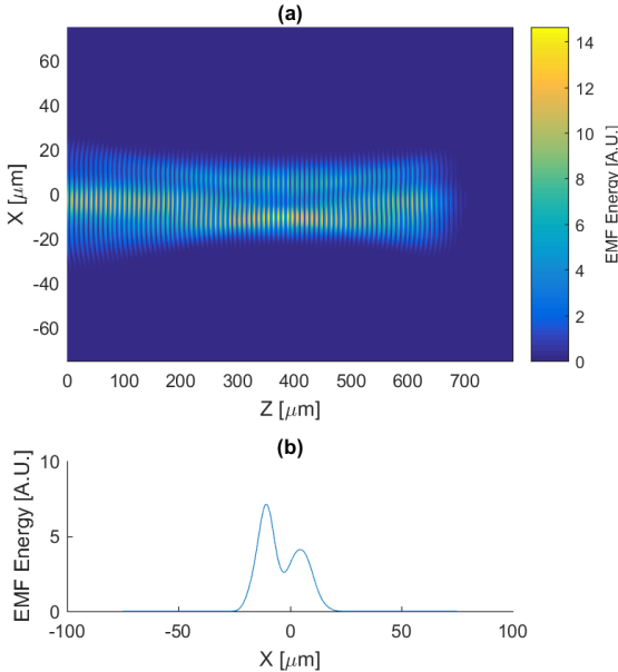
FIG. 9: Simulated intensity profile of imperfect beam in vacuum. (a) The spatially resolved electromagnetic energy of the vacuum simulation is shown after 2.5 ps in (a). A lineout at Z = 392 \mu\text{m} was taken and is plotted in (b). As can be seen, the simulation did not successfully capture the fitted spot shown in Figure 8, but instead generated two broad peaks at focus.
