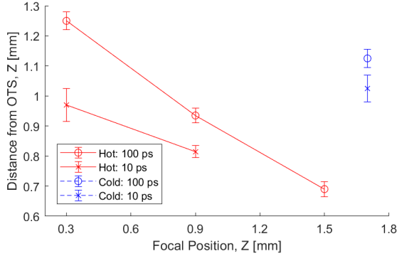
FIG. 4: Channel penetration. The final distances from the original target surface (OTS) are plotted against the vacuum focal position for the 100 ps and 10 ps in both the hot and cold plasmas. Deeper penetration would therefore have a lower value. These measurements were made using the 4\omega probe.
