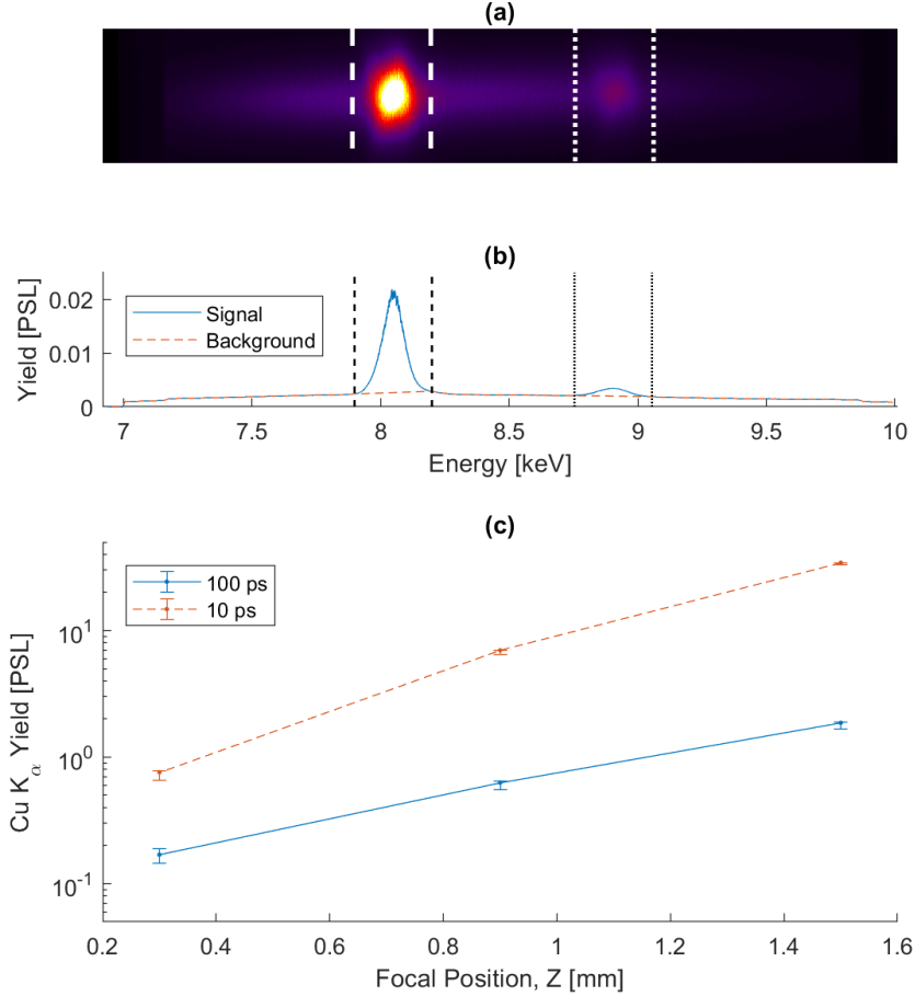
FIG. 16: Von Hamos spectrometer output and Cu K_{\alpha} yield. An example von Hamos spectrometer signal is shown in (a) with white dashed lines indicating the Cu K_{\alpha} region and dotted lines indicating the Cu K_{\beta} region. An integrated lineout is shown in (b) along with the background profile. The K_{\alpha} region was then integrated within a 0.15 keV range of its peak to calculate the total Cu K_{\alpha} yield plotted in (c) for each hot plasma shot.
