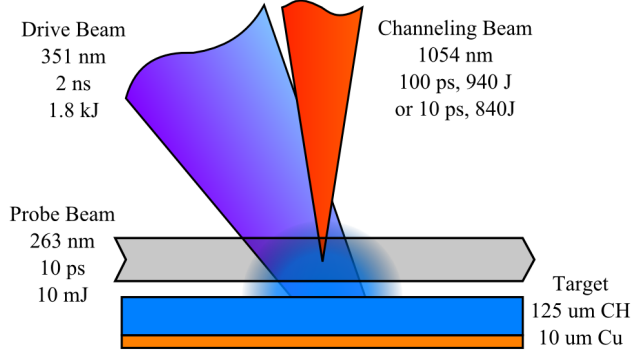
FIG. 1: Schematic of experimental setup. A 3\omega drive beam ablates the surface of a plastic target, generating a plasma plume. Upon completion of the driving phase, a 1\omega channeling pulse begins propagation through the plasma normal to the target’s surface. A 4\omega probe pulse is used to observe the resulting channel formations.
