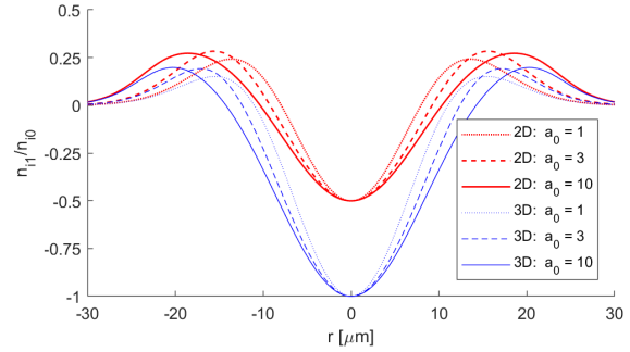
FIG. 13: Integration of channeling profile equation at various intensities. Equation 1 was integrated until the 3D density profile was fully evacuated at various intensities. Red (thick) lines indicate the integration was performed in 2D while blue (thin) lines indicate 3D. Dotted lines correspond to a_0 = 1 at t = 3.758 ps, dashed lines to a_0 = 3 at t = 1.732 ps, and solid lines to a_0 = 10 at t = 0.907 ps.
