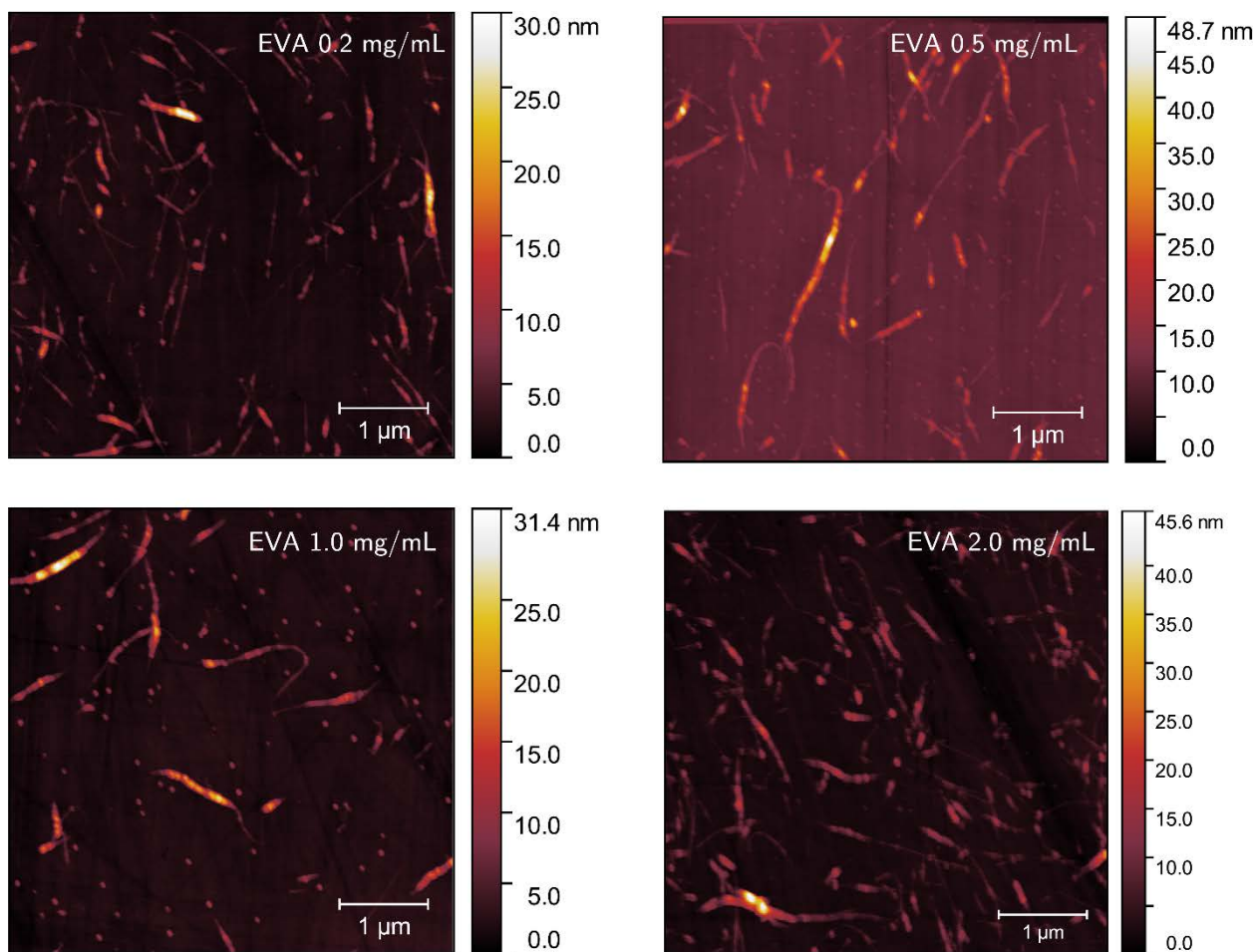
Figure S5 AFM images of diluted EVA/SWCNT nanohybrids on glass obtained from different EVA polymer concentrations (indicated in the top-right corner of each map). In all the four images it is possible to observe individual SWCNTs.
