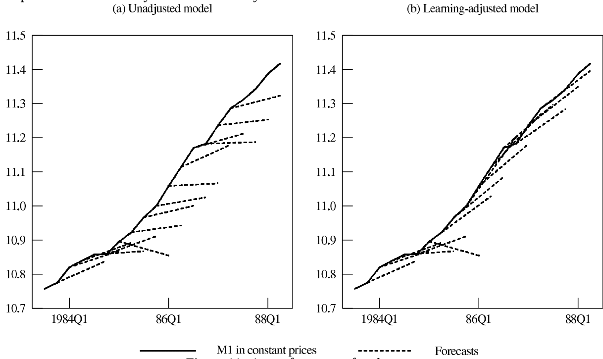
Figure 11: 4-step forecasts of real money
