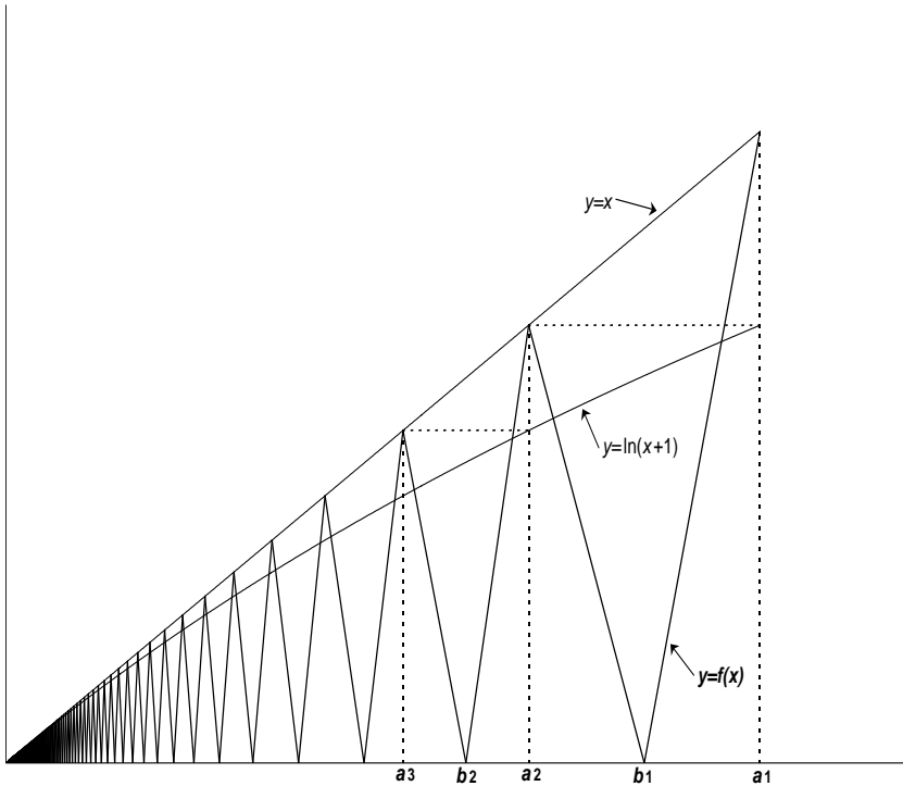
Fig. 1. The construction of y = f(x) over [0, 1]
