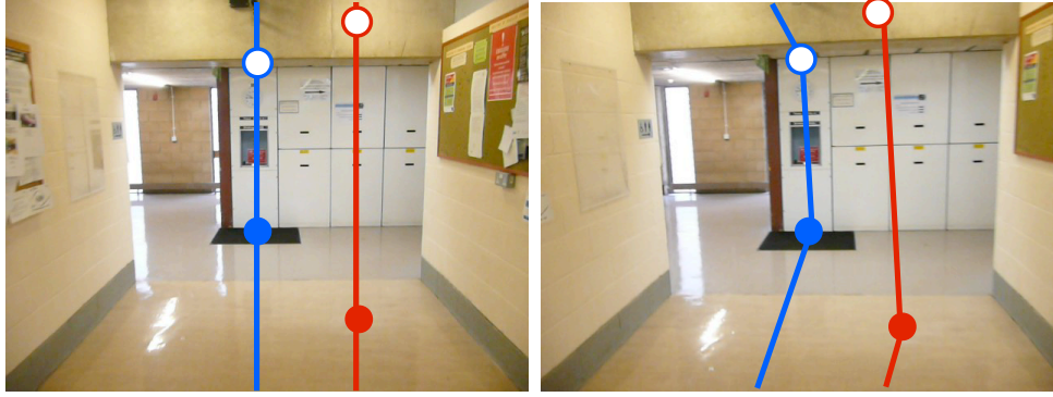
Figure 6.4: Two hypotheses for the location of the seam and the reprojections they imply for each image column in an auxiliary image. The blue dot happens to be a correct hypothesis (unknown to the system), while the red dot is incorrect. As a result, the blue line corresponds to the same set of 3D locations in both images but the red line does not.
