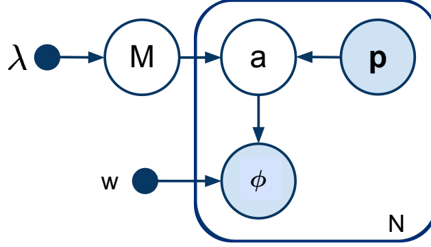
Figure 6.2: The graphical model relating scenes M to monocular image features \phi . \mathbf{p} = (x, y) is a pixel location and a is the orientation predicted (deterministically) by M at \mathbf{p} .
