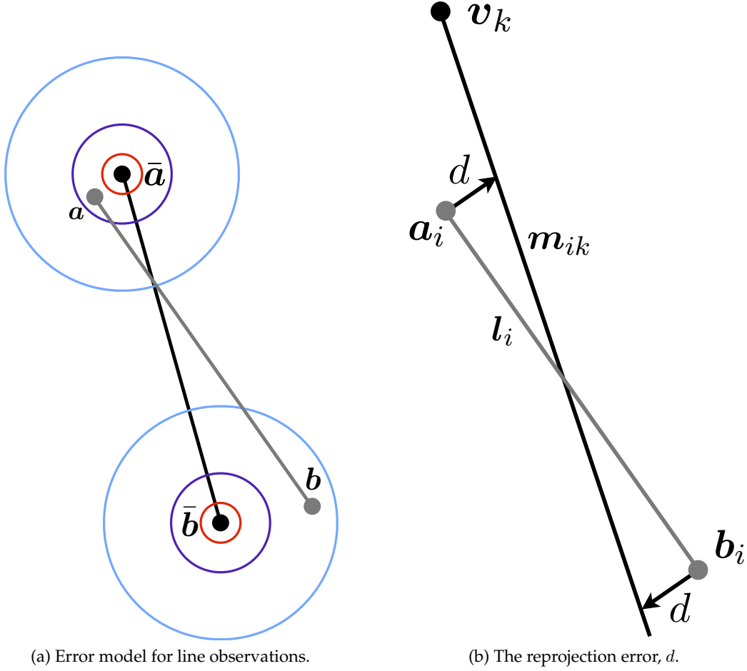
Figure 5.2: Illustration of our error model and various geometric quantities involved in the derivations in the main text.
