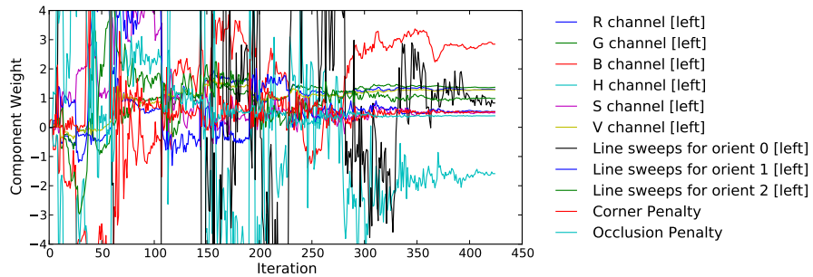
(d) Evolution of f_{\text{labelling}}^{\text{sview}} during training (selected features only)
