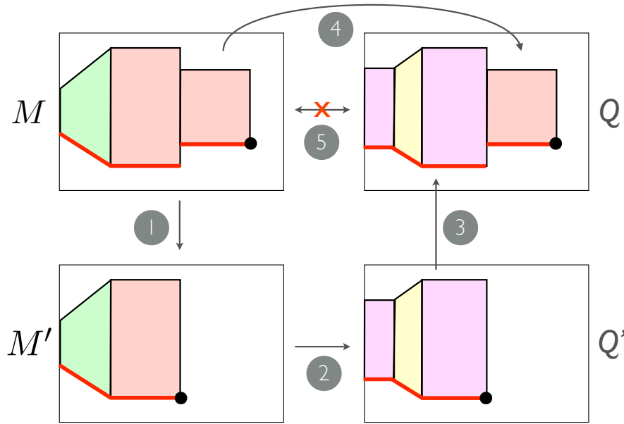
Figure 6.14: A graphical sketch of the proof of Theorem 1. The proof proceeds counter-clockwise from top left. First we let M be an optimal scene for some sub-problem, then (1) define M' to be its truncation. We then (2) postulate some Q' with value greater than M' , and then from this we (3,4) construct Q . The contradiction follows by (5) comparing M and Q .
