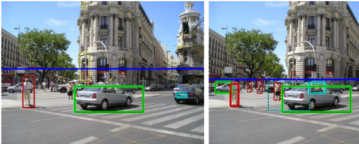
Figure 2.3: The left image shows car and pedestrian detections when using local features only. The right image shows detections when geometric context is leveraged: several false-positives are eliminated and several new correct detections are made. Reprinted with express permission of Dr Derek Hoiem.
