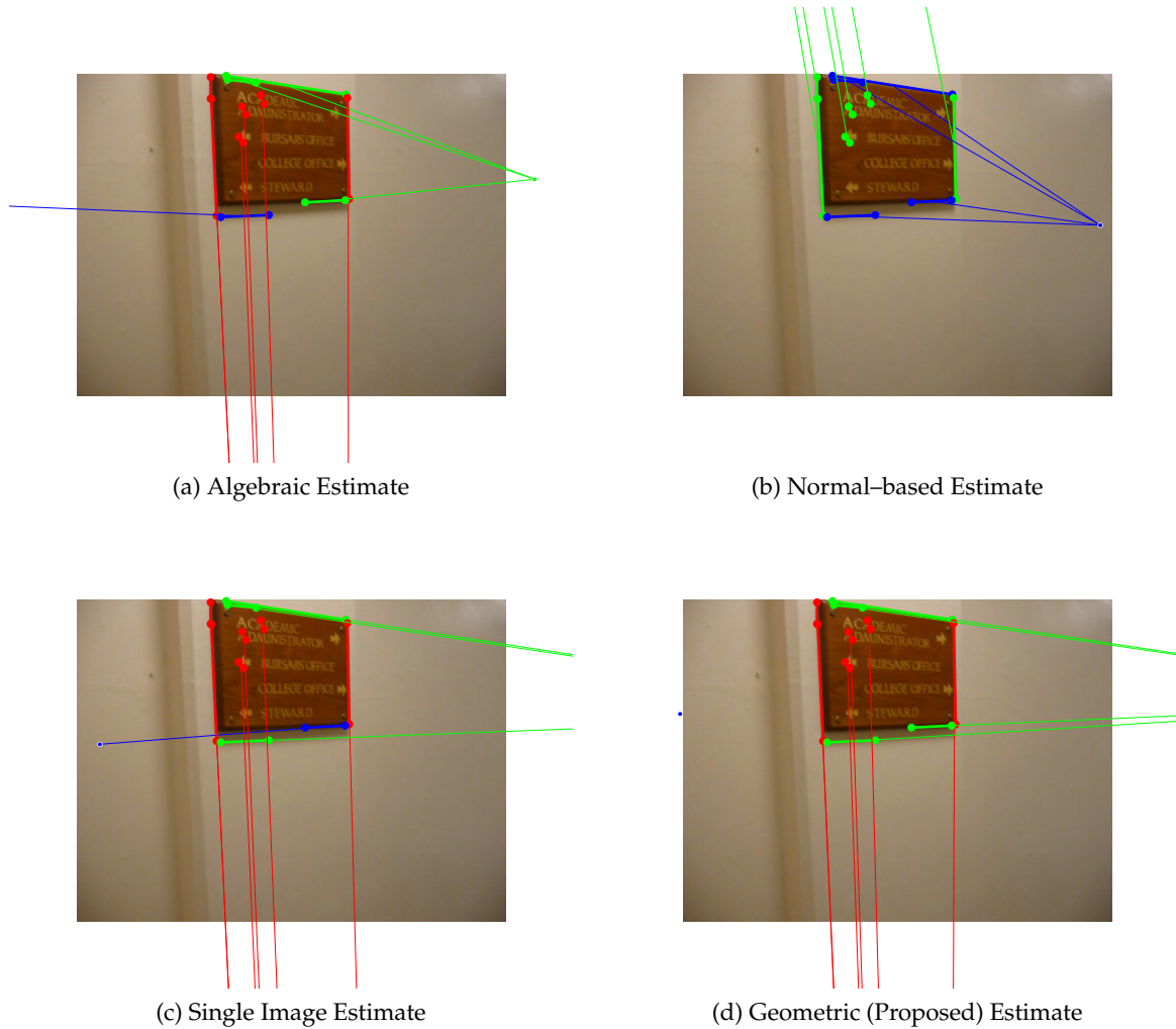
Figure 5.5: Comparison of rotation estimation algorithms for an example drawn from the “Bursary” sequence. Though only one frame is shown here, each algorithm other than (c) was provided with 7 input frames.
