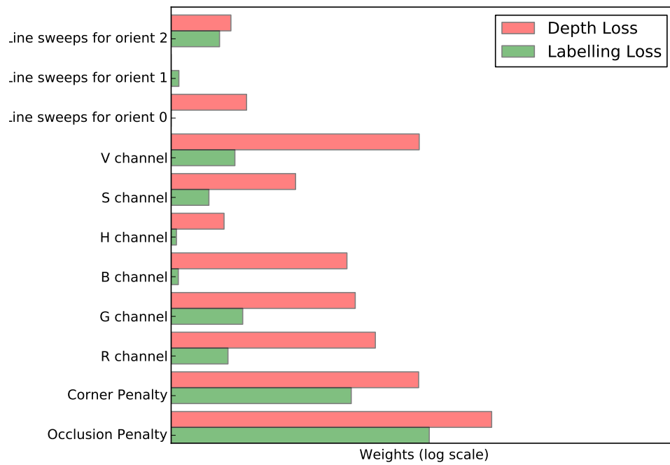
(a) Weight vector learned for single view features
