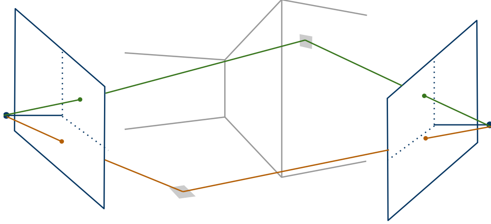
Figure 6.3: Pixel correspondences across multiple views are computed by back-projection onto the model M followed by re-projection into auxiliary views.
