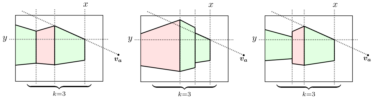
Figure 6.13: Three models satisfying the sub-problem \text{Best}(x, y, o) .
