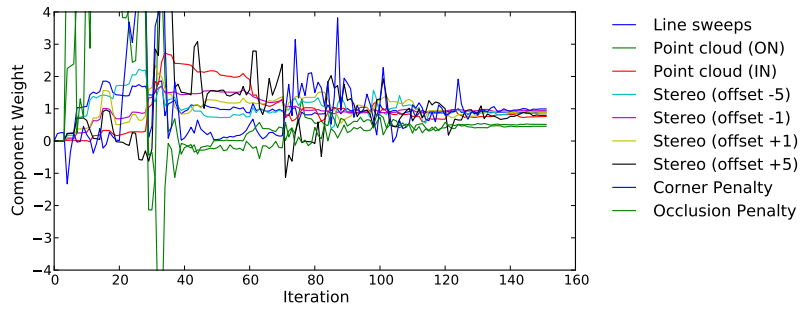
(b) Evolution of f_{\text{labelling}}^{\text{mview}} during training
