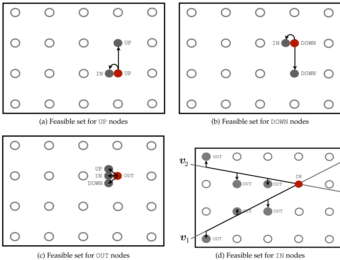
Figure 6.15: The feasible sets for each of the four new node labels introduced in Section 6.4.4. Each panel highlights one node and shows the outgoing edges for just that node. These are repeated for every pixel and orientation.
