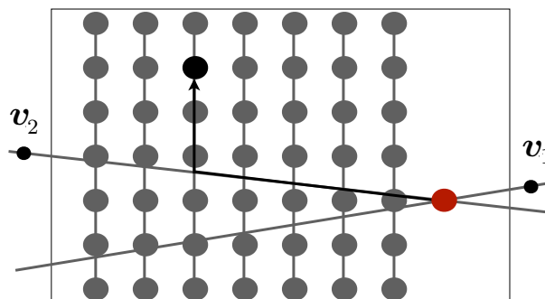
Figure 6.12: The search graph corresponding to the second version of our dynamic programming algorithm (Section 6.4.2). Here we have highlighted a single node (red circle), which has outgoing edges to every pixel to its left (grey circles). One neighbouring state (black dot) is singled out to show that the edges between states represents displacement along a vanishing direction followed by displacement in the vertical direction.
