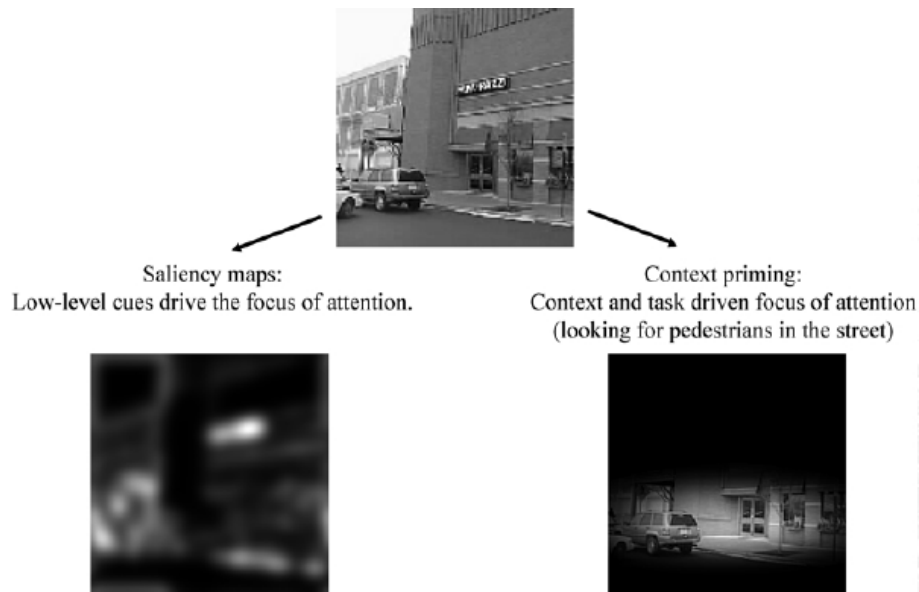
Figure 2.1: Torralba et al. [67] is able to improve upon traditional interest point detectors by learning the relationship between gist features and likely object locations. Reprinted with express permission of Prof Antonio Torralba.
