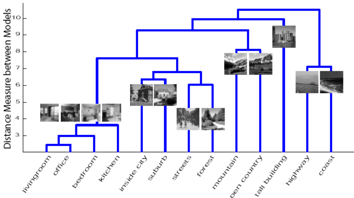
Figure 2.2: Dendrogram showing the relationships between scene categories learnt by the system of Fei-Fei and Perona [18]. The model matches human intuition well. Reprinted with express permission of Prof Fei-Fei Li.
