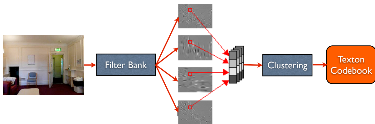
Figure 3.1: The texton generation process.
