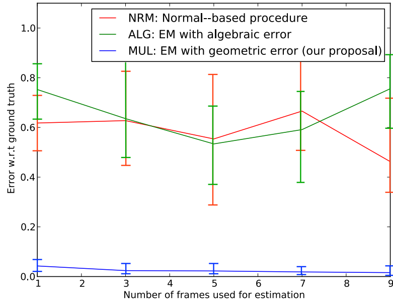
(a) Estimation error versus number of input frames.
