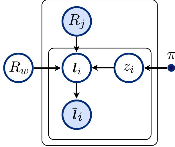
Figure 5.1: A graphical model relating line segments to vanishing points.
