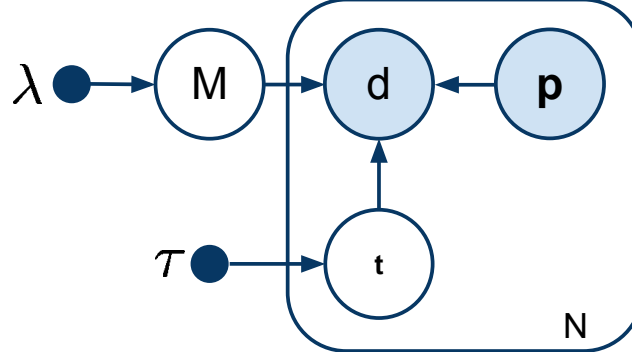
Figure 6.5: The graphical model relating indoor Manhattan models to 3D points. The hidden variable t indicates whether the point is inside, outside, or coincident with the model.
