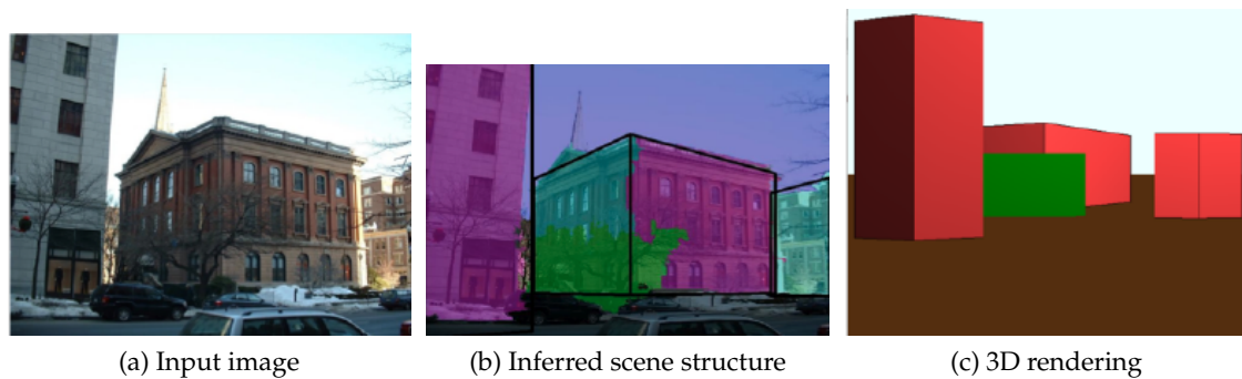
Figure 2.8: Results from the blocks world model of Gupta et al. [28]. Reprinted with express permission of Dr Abhinav Gupta.
