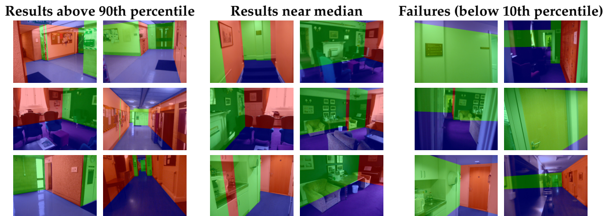
Figure 6.18: Scenes output from our system. The left column shows results above the 90th percentile of performance (relative depth error), the middle column shows results near median performance, and the right column shows failure cases.
