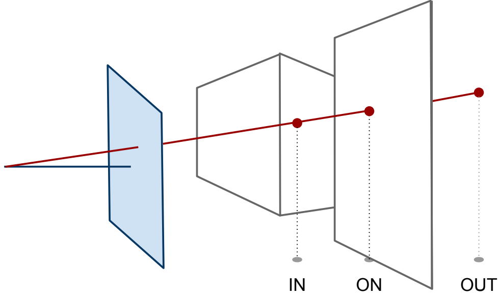
Figure 6.6: Depth measurements d_i might be generated by a surface in our model (represented by t_i = \text{ON} ) or by an object inside or outside the environment (in which case t_i = \text{IN}, \text{OUT} respectively).
