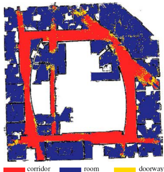
Figure 2.11: Semantic labels assigned by the range data classification system of Martinez et al. [51]. 82% of places were correctly classified, despite the environment not having been seen during training. Reprinted with express permission of Dr Oscar Martinez Mozos.
