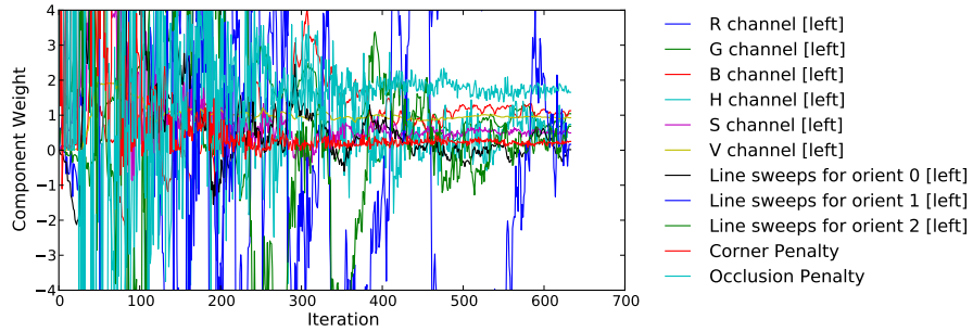
(c) Evolution of f_{\text{depth}}^{\text{sview}} during training (selected features only)
