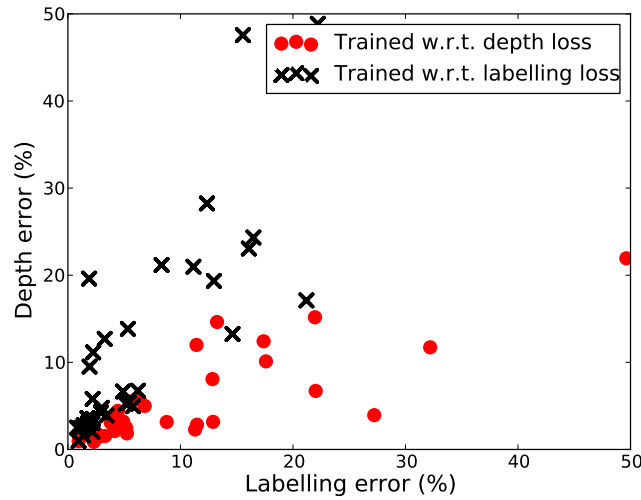
Figure 7.1: The effect of the loss function on training. We train two predictors, one with respect to \Delta_{\text{depth}} and one with respect to \Delta_{\text{labelling}} , then evaluate both on all held-out instances. Each data point shows the error obtained by one predictor on one held-out instance. The differing distribution of errors shows that the two predictors trade off errors as expected.
