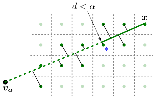
Figure 6.16: Each time we evaluate an \text{IN} node we walk along a vanishing line from some state x to a vanishing point v (green line), examining each state we encounter (green dots). The approximation described in Section 6.4.5 permits us to terminate this search when we first encounter a node within a threshold distance of the line (blue asterisk).
