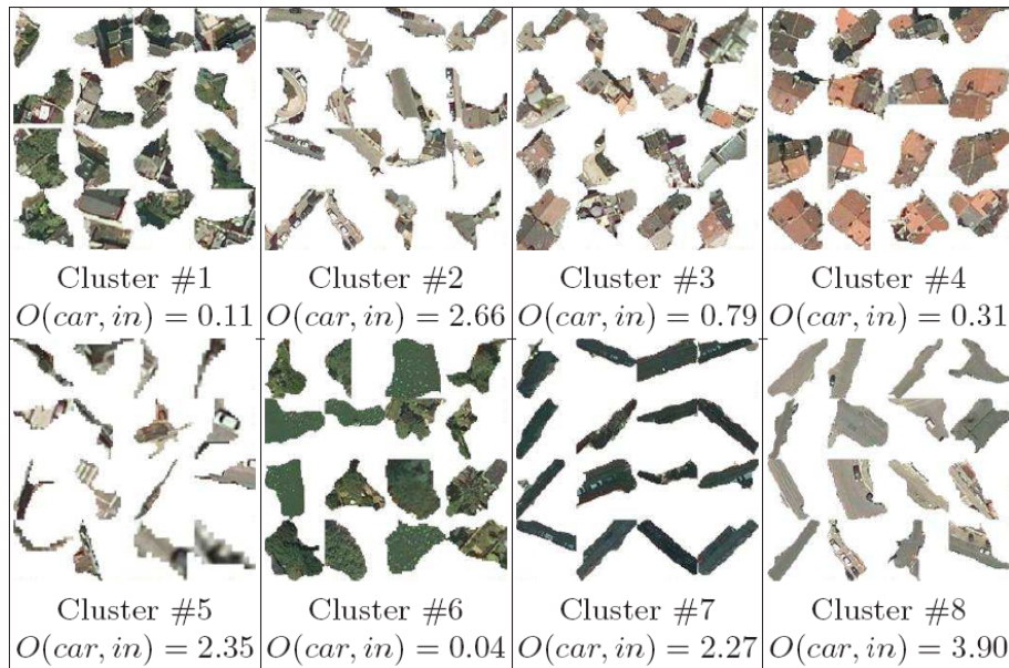
Figure 2.10: Superpixels clusters generated by the model of Heitz and Koller [32]. Shown below each panel is the odds ratios for a car appearing near a superpixel from that class. The odds ratio is higher for road-like regions than for foliage- or water-like regions. Reprinted with express permission of Prof Daphne Koller.
