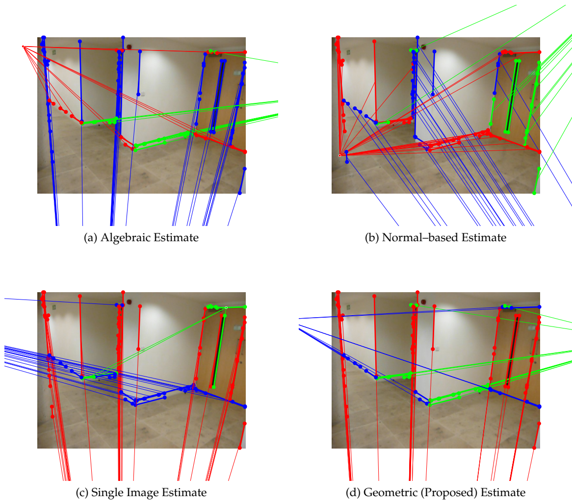
Figure 5.7: Comparison of rotation estimation algorithms for an example drawn from the “Ground1” sequence. Though only one frame is shown here, each algorithm other than (c) was provided with 7 input frames.
