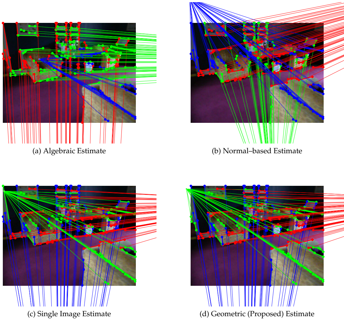
Figure 5.6: Comparison of rotation estimation algorithms for an example drawn from the “MCR” sequence. Though only one frame is shown here, each algorithm other than (c) was provided with 7 input frames.
