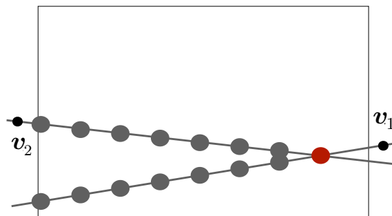
Figure 6.8: The search graph corresponding to the first version of our dynamic programming algorithm. This figure identifies one node (red circle) and shows all neighbours to which it is connected via outgoing edges (grey circle).
