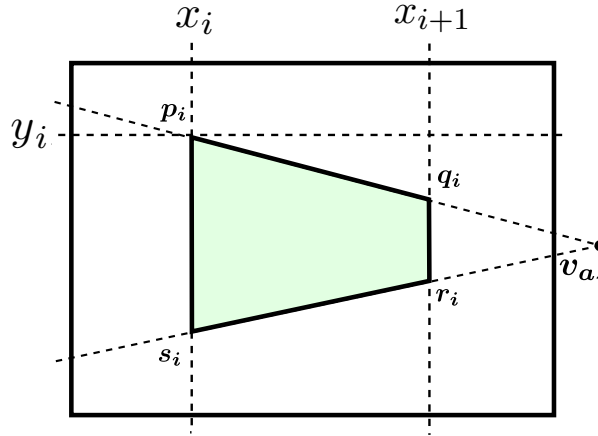
Figure 4.4: The scalars x_i, x_{i+1}, y_i , together with the vanishing point index o_i \in \{1, 2\} and the homology H_a fully determine the four vertices of a wall.
