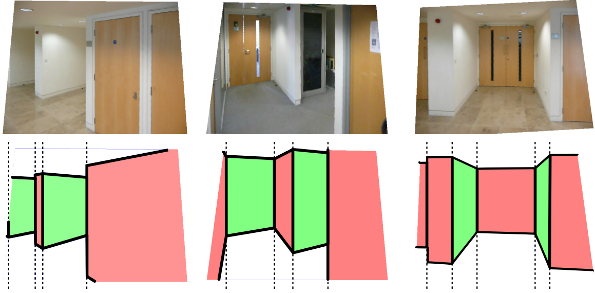
Figure 4.3: Three input images and the indoor Manhattan models we seek. Notice how each image column intersects exactly one wall.
