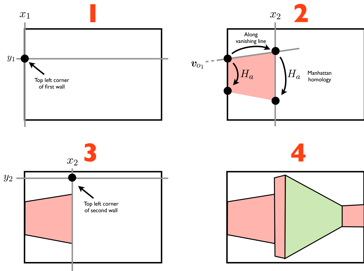
Figure 4.5: The meaning of the parameters in the vertex representation is illustrated through a constructive example. (1) The top-left corner of the first wall is at (x_1, y_1) . (2) The top-right corner of the first wall is found by intersecting the vanishing line with the line x_2 . Then both points are projected through H_a , yielding the four corners of the first wall. (3) The top-left corner of the second wall is at (x_2, y_2) . (4) This is repeated to build up the entire model.
