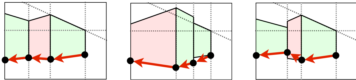
Figure 6.11: Three paths through the search graph after making the changes described in Section 6.4.2 to permit occluding corners. The two right-most scenes cannot be represented in the previous search graph. Note that there is a state at the bottom-right of each wall segment.
