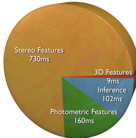
Figure 6.17: Processing time for feature computation and inference in our system, averaged over all evaluation instances. The mean total processing time was 997ms.
