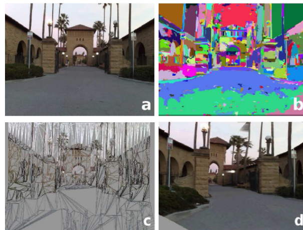
Figure 2.4: Results from the geometric context system of Saxena et al. [58]. From top left to bottom right the panes show (a) the original, (b) the superpixels, (c) the inferred 3D model, (d) a re-projection of the 3D scene. Reprinted with express permission of Dr Ashutosh Saxena.
