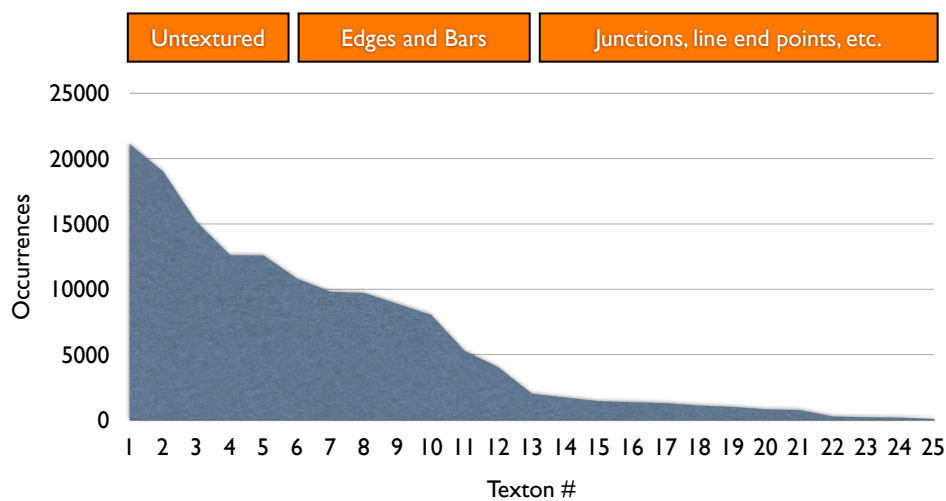
Figure 3.4: Frequency distribution of textons. The texton generation process assigns more textons to describing salient but rare image structures such as junctions and line end points than it assigns to frequent but non-discriminative image regions such as textureless patches.
