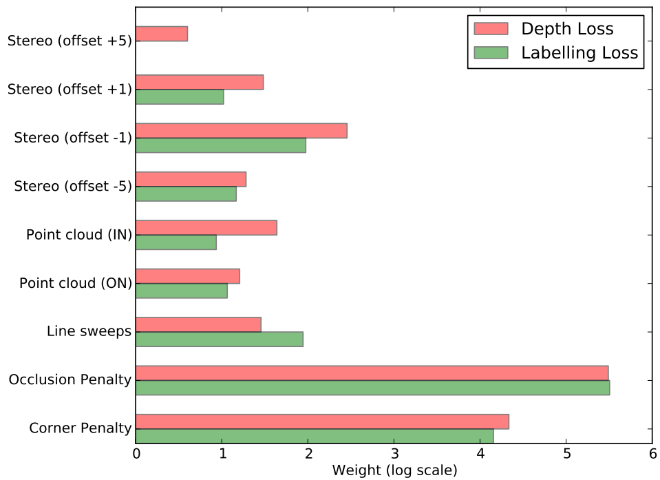
(b) Weight vector learned for multiple view features
