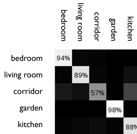
Figure 3.7: Confusion matrix for place recognition. This figure corresponds to the bottom row of Table 3.1.
