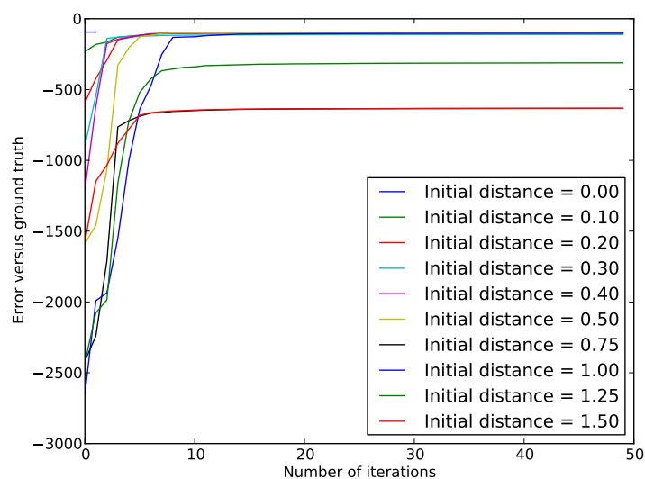
(b) Convergence of log-likelihood
