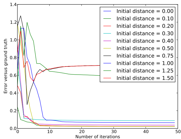
(a) Convergence of error (with respect to ground truth)
