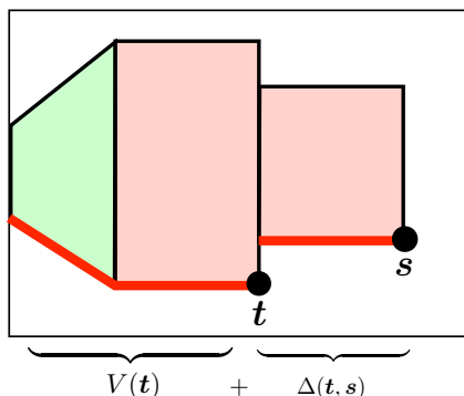
Figure 6.10: The computation of the value function at s . This figure shows just one term in the maximisation (6.52); computing V(s) involves maximisation over all possible states t .
