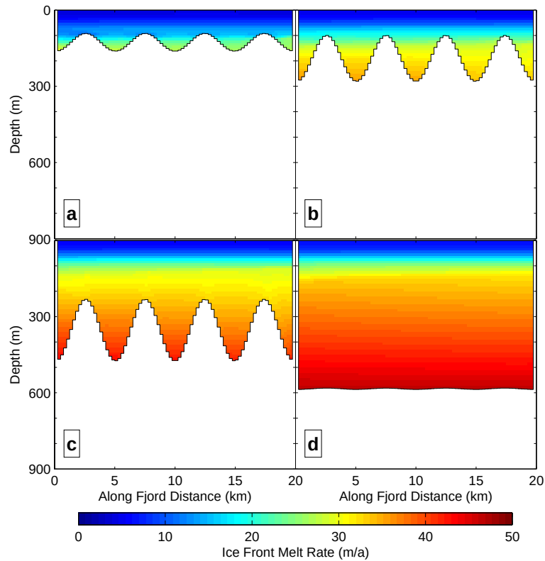
Figure 5.27: Ice front melt rates (m/a) for ice shelves of length a) 30 km, b) 20 km, c) 10 km and d) 0.5 km. Melt rates are plotted looking out of the fjord.
