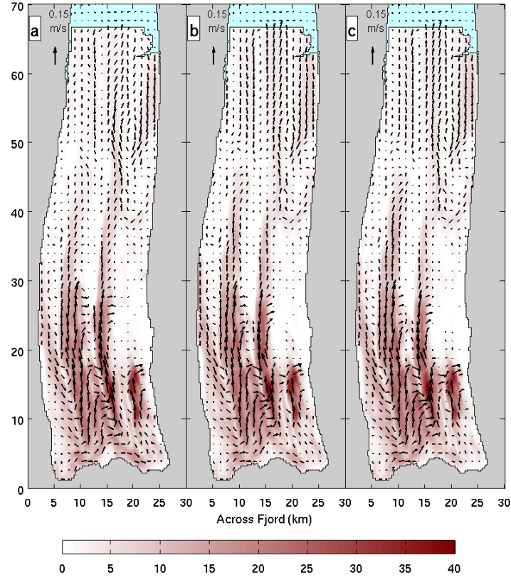
Figure 6.3: Melt rates (m/a) and sub-ice layer velocities (m/s) for the a) small-basin, b) linear-sloping and c) large-basin bathymetries.
