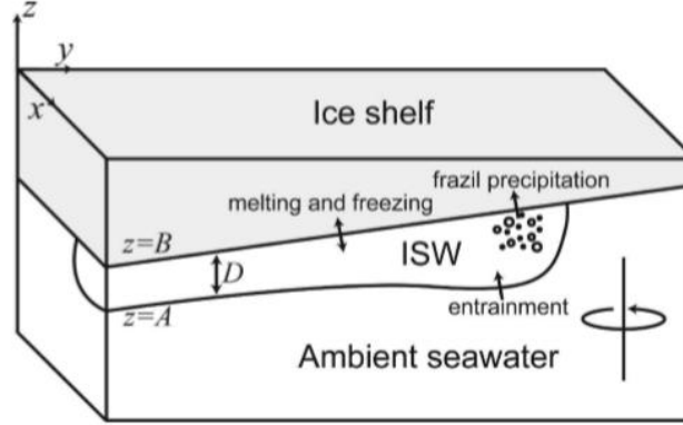
Figure 3.1: Schematic of a layer of meltwater (ISW) between a floating ice shelf and ambient seawater. Relevant processes (melting, freezing and entrainment) along with co-ordinates used in equations 3.1 and 3.2 are shown (Source: Holland and Feltham (2006) ).
