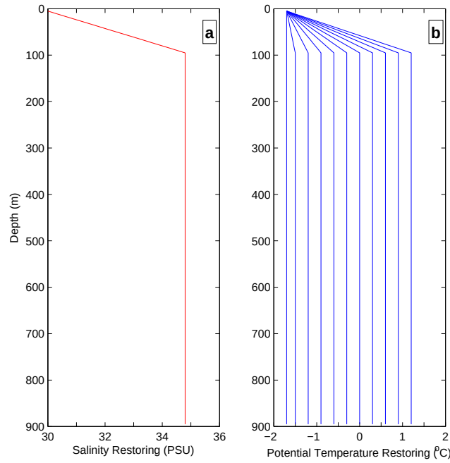
Figure 5.16: a) Salinity and b) potential temperature restoring profiles for the eleven warming and cooling scenarios.
