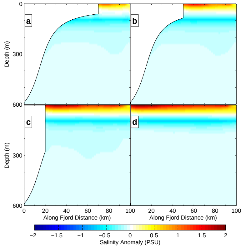
Figure 5.24: Salinity anomaly section along the central keel for ice shelves of length a) 70 km, b) 50 km, c) 20 km and d) 0.5 km.
