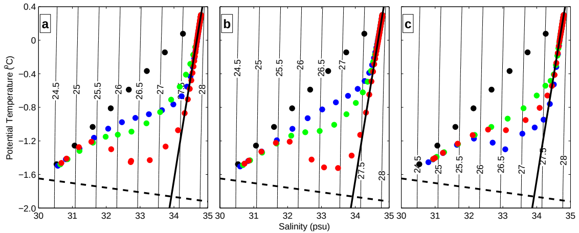
Figure 4.5: \Theta - S space for the a) 0-, b) 2- and c) 8-channel configurations. The solid black line represents the Gade line with gradient 2.77 °C/PSU and the dashed black line represents the freezing temperature. Contours are density contours (density -1000kg/m 3 ) separated by 0.5kg/m 3 . The profiles are taken in the same location as the four channel configuration and their locations are denoted by the coloured dots in Figure 4.2.
