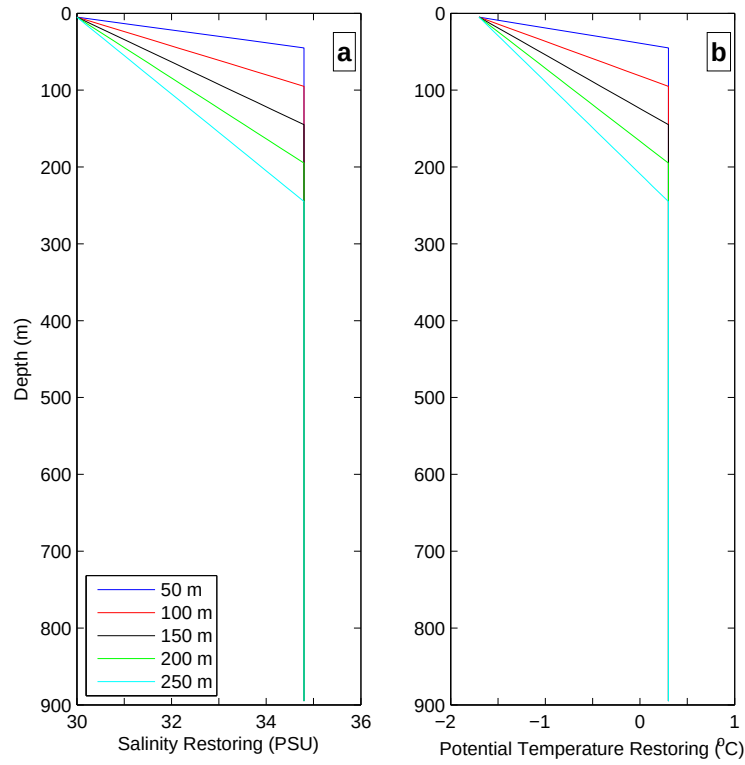
Figure 5.1: a) Salinity and b) Potential Temperature profiles used as initial conditions and restoring at the northern boundary for stratification depths of 50 m (dark blue), 100 m (red), 150 m (black), 200 m (green) and 250 m (cyan).
