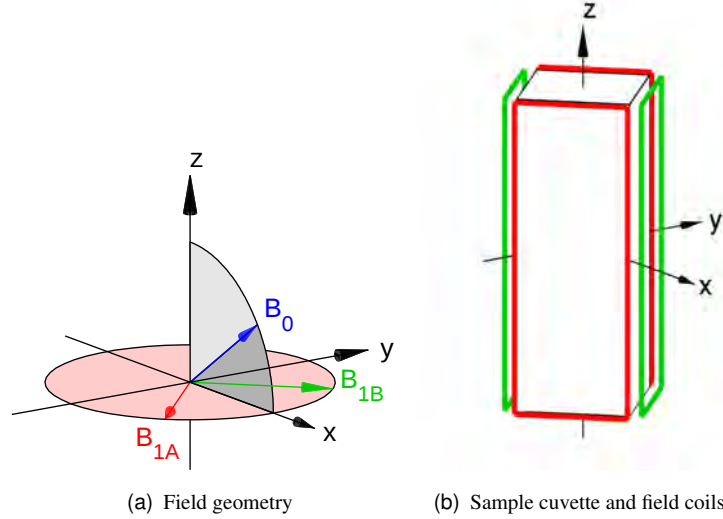
Figure 5.1: Figures illustrating the field geometry. The static field B_0 is applied in the xz -plane at an angle \theta to the x -axis. For linearly polarised RF ( \phi_{rf} = 0 ) this means that \theta = 0 gives parallel RF and static fields, whilst \theta = \pi/2 gives perpendicular RF and static fields; this convention matches that used in Chapter 4. The RF field is applied through two pairs of field coils, marked in red and green. By adjusting the phase difference \phi_{rf} between the two coils, linearly or circularly polarised fields may be generated in the xy -plane. In the experimental measurements, these coils are 12 mm \times 5 mm rectangular loops, separated by 5 mm.
