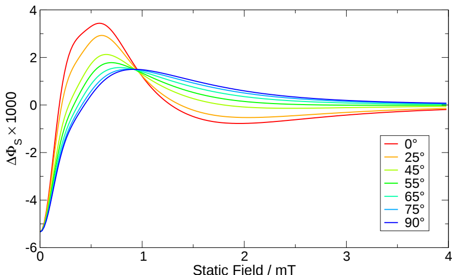
Figure 4.11: Approximate, simulated low-field optically detected EPR spectra of [\text{Py-d}_{10}^+ \text{1,3-DCB}^{\bullet-}] at a radio frequency of 5 MHz. The simulations were performed by treating the RF field as invariant during a radical pair lifetime. Values of \theta are as indicated. B_1 = 0.3 \text{ mT} and k = 4 \times 10^7 \text{ s}^{-1} . The full time-dependent calculation for these parameters is shown in Figure 4.10(b).
