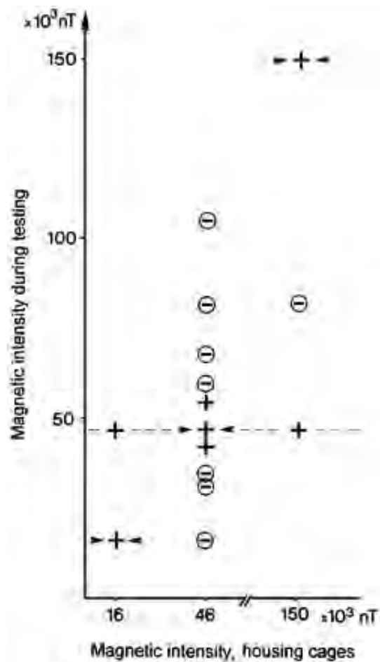
Figure 6.10: European robins housed in a 46\mu\text{T} field ( i.e. the geomagnetic field at Frankfurt) become disoriented if tested in fields greater than 60\mu\text{T} or smaller than 34\mu\text{T} . Acclimatisation allows the magnetic compass sense to operate over a wider range of field strengths. “+” denotes successful orientation and \ominus disorientation. Figure from [302]. With kind permission of Springer Science+Business Media.
