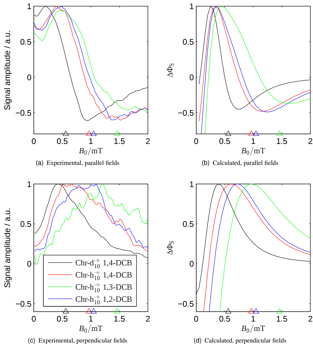
Figure 4.5: Left: Experimental MARY- \nu spectra measured in four isomer/isotopomer variants of the [\text{Chr}^+ \text{DCB}^{\bullet-}] radical pair at \nu_{\text{rf}} = 5 \text{ MHz} . Right: Corresponding simulations made with \gamma -COMPUTE using B_1 = -\omega_1/\gamma_e = 100 \mu\text{T} , \nu_{\text{rf}} = 5 \text{ MHz} , exponential model rate constant k = 5.6 \times 10^7 \text{ s}^{-1} and n = 64 . Hyperfine coupling constants are given in Table 4.1. All plots have been scaled to the same maximum intensity because the different exciplexes have different intensities. Overall effective HFCs from Table 4.1 are marked with small triangles for each system.
