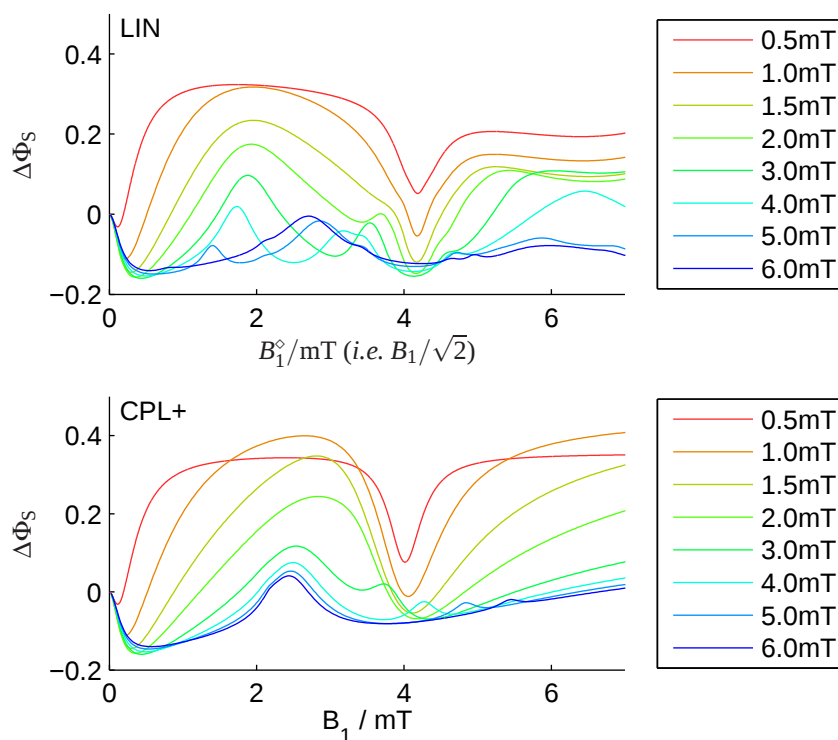
(a) B_1 plots for “1–0” RPs having a single spin- \frac{1}{2} whose HFC is given in the legend.
