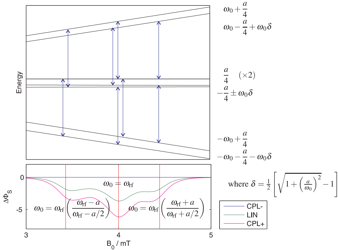
Figure 5.21: Expanded view of the energy levels (top) and MARY-v spectra (bottom) for a RP that contains a single spin- 1/2 nucleus. The same RP was used in Figure 5.20. Parameters: \nu_{rf} = 112 MHz, B_1 = 0.1 mT, a = 1.0 mT, n = 64 , \theta = \pi/2 and k = 2.8 \times 10^7 s ^{-1} . Energies corresponding to absorption or emission of an RF photon are shown by vertical lines. The three peaks in the MARY-v spectrum are marked with their positions calculated using first order perturbation theory for a weak RF field. It is clear that they form a singlet and a distorted doublet.
