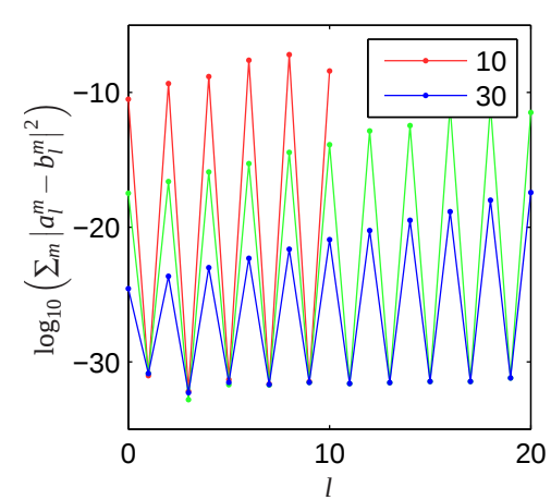
(d) Static field B_0 = 50 \mu\text{T} . Differences between the SolveInvL SphHReps a_l^m and converged PyDMAFST b_l^m .
