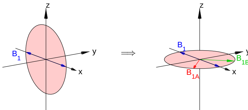
Figure 5.33: Geometrical relationship between (a) CPL \pm , RMS strength B_1 , \theta = 0 ; (b) LIN, RMS strength B_1/\sqrt{2} , \theta = \pi/2 ; and (c) CPL + , RMS strength B_1/2 , \theta = \pi/2 . Left: (a) \rightarrow (b). Right: (b) \rightarrow (c). See text for details.
