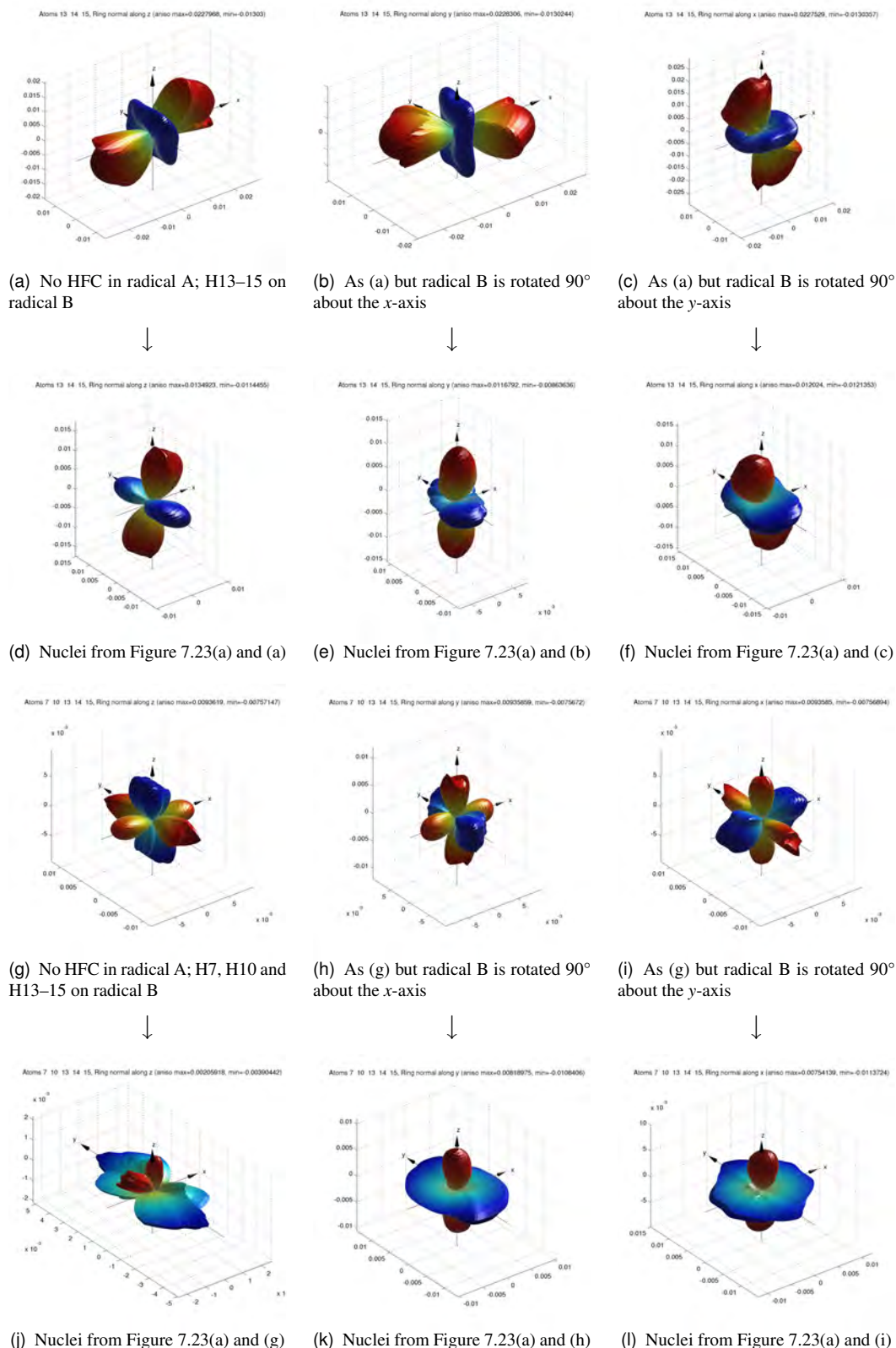
Figure 7.24: Do hyperfine anisotropies in “m–0” and “0–n” RPs add when the radicals are combined to form an “m–n” RP? Calculations are performed for the [FAD^{\bullet-} Y^{\bullet}] RP ( i.e. A is FAD^{\bullet-} and B is Y^{\bullet} ) with B_0 = 50 \mu T and k = 2 \times 10^5 s^{-1} (equivalent to a RP lifetime of 5 \mu s ). The atom numbering scheme and hyperfine tensors used are shown in Figures 7.17 and 7.18.
