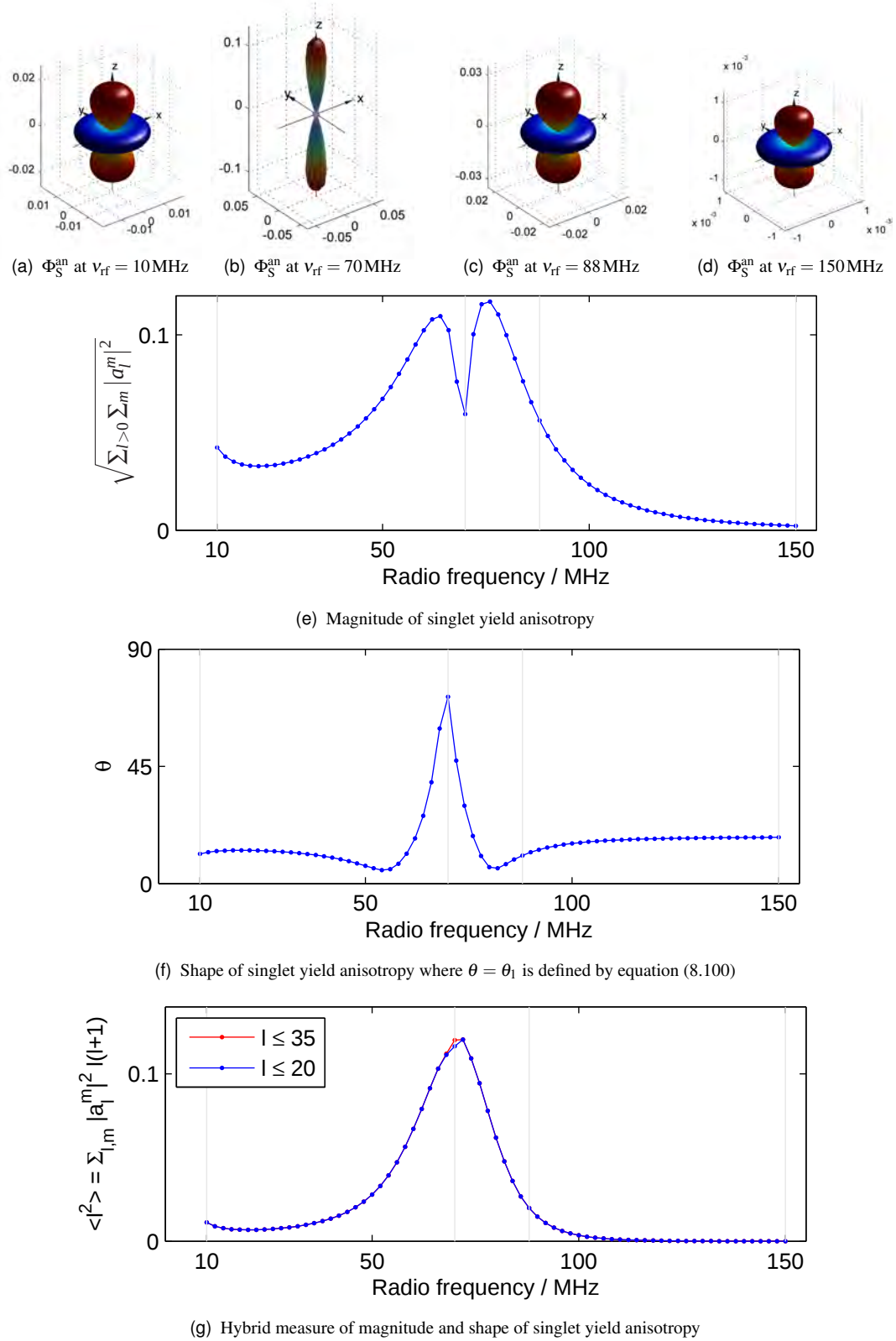
Figure 8.20: Effect of radio frequency \nu_{\text{rf}} on singlet yield. Calculations were performed in a one-proton RP model system using the gCOMPFAST algorithm with B_1 = 100 \mu\text{T} , k = 2 \times 10^5 \text{ s}^{-1} , HFC a = 2.5 \text{ mT} , \alpha = 12.5 \mu\text{T} , \beta = 0 , n = 128 , and \text{MaxL} = 35 . Figures (a–d) show singlet yield anisotropies at the \nu_{\text{rf}} values marked with grey vertical lines.
