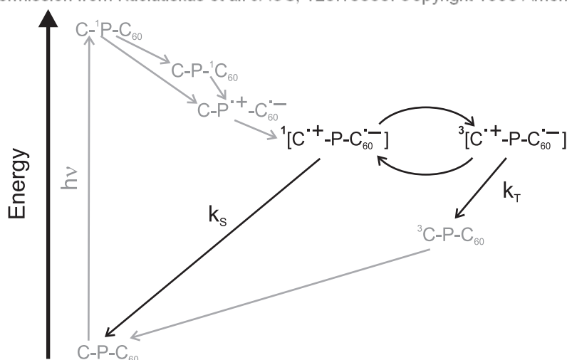
Figure 8.23: Carotenoid-porphyrin-fullerene model compound \text{CPC}_{60} .
