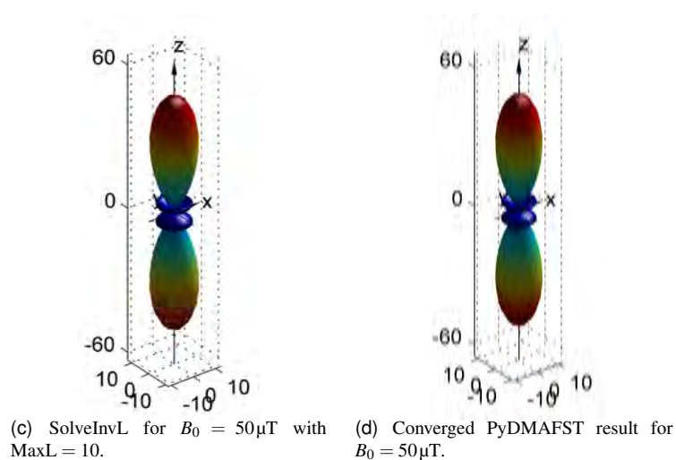
Figure 8.9: Polar plots of 1000 \times singlet yield anisotropy to accompany Figure 8.8. Calculations were made in a one-proton RP using the CalcSphHRep code and the following parameters: k = 2 \times 10^6 \text{ s}^{-1} , a = 2.5 \text{ mT} , \alpha = 12.5 \mu\text{T} and \beta = 0 \mu\text{T} .
