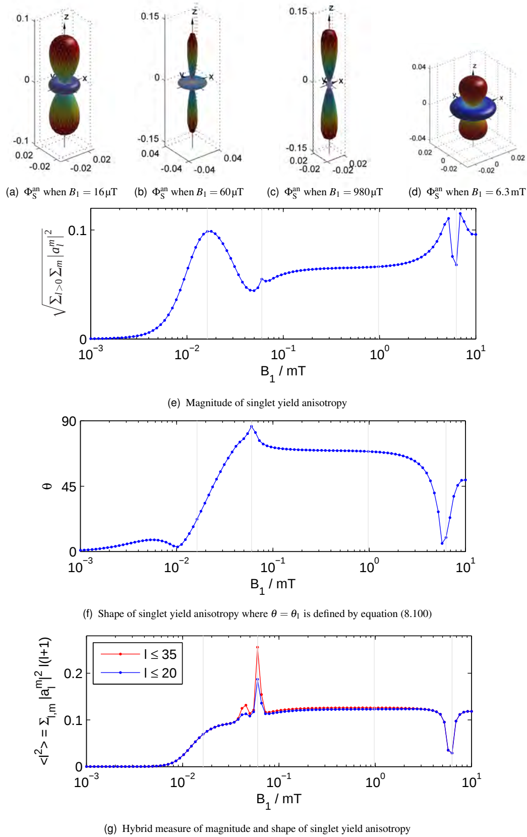
Figure 8.18: Effect of B_1 on singlet yield. Calculations were performed in a one-proton RP model system using the gCOMPFAST algorithm with k = 2 \times 10^5 \text{ s}^{-1} , B_0 = 0 \text{ mT} , HFC a = 2.5 \text{ mT} , \alpha = 12.5 \mu\text{T} , \beta = 0 , n = 128 , \nu_{\text{rf}} = 2.5 \times 28 = 70 \text{ MHz} , and \text{MaxL} = 35 . Figures (a–d) show singlet yield anisotropies at the B_1 values marked with grey vertical lines.
