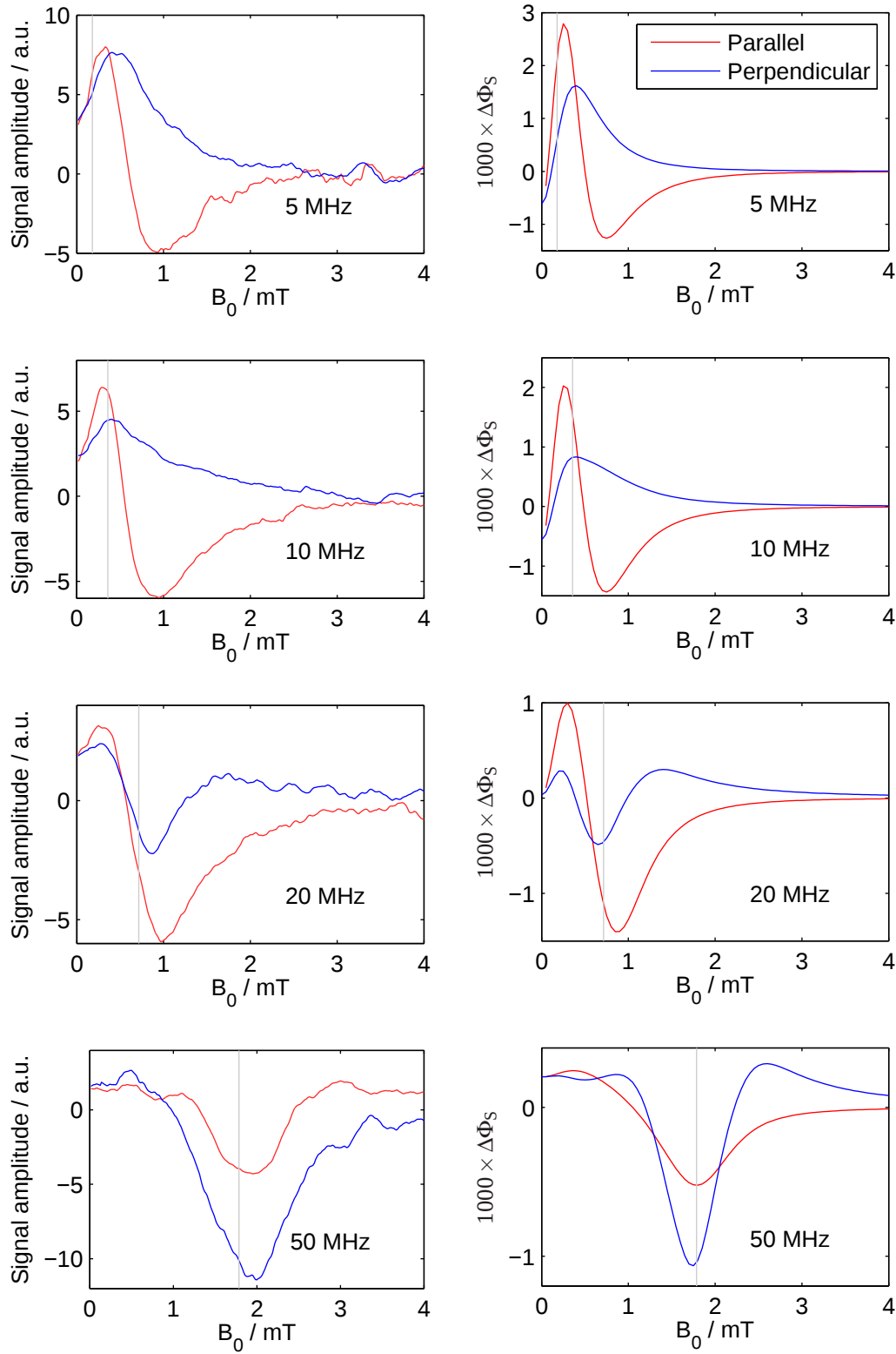
Figure 4.4: Left: Experimental MARY-v spectra measured in the [\text{Chr-d}_{12}^{*+} \text{1,4-DCB}^{*-}] radical pair. The frequency \nu_{\text{rf}} of the RF field is indicated for each spectrum. Right: Corresponding simulations made with \gamma -COMPUTE using B_1 = -\omega_1/\gamma_e = 100 \mu\text{T} , exponential model rate constant k = 5.6 \times 10^7 \text{ s}^{-1} and n = 64 . Hyperfine coupling constants are given in Table 4.1. Grey vertical lines show the static field at which a Zeeman resonance might be anticipated ( B_0 = -2\pi\nu_{\text{rf}}/\gamma_e ).
