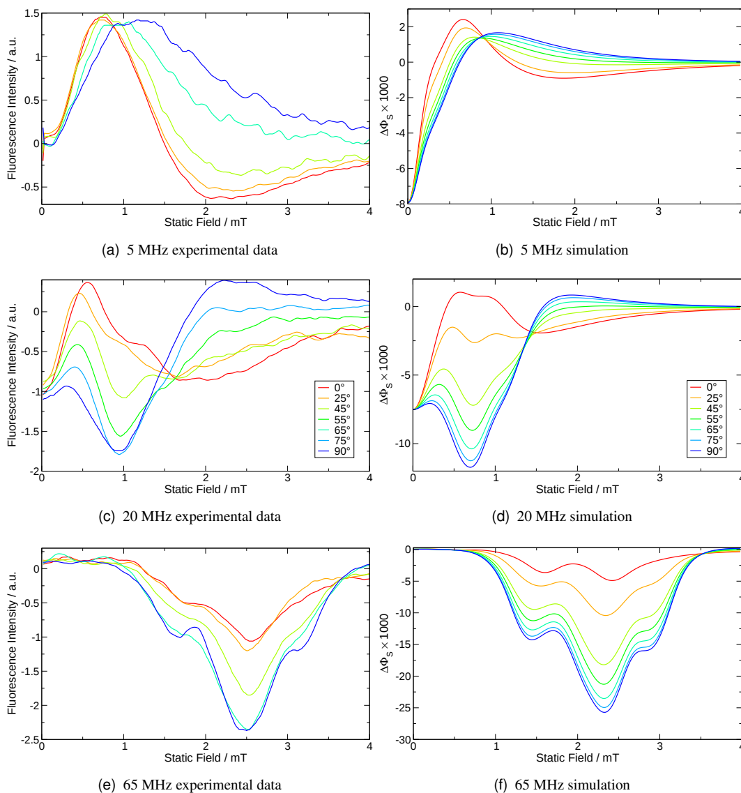
Figure 4.10: Experimental (left) and simulated (right) low-field optically detected EPR spectra of [\text{Py-d}_{10}^+ \text{1,3-DCB}^-] at radio frequencies of \nu_{\text{rf}} = 5 \text{ MHz} (top), 20 \text{ MHz} (centre) and 65 \text{ MHz} (bottom). Values of \theta are as indicated in the legend. The same colours are used for all plots, even though experimental data were not collected for some combinations of \nu_{\text{rf}} and \theta . The simulations were performed using B_1 = 0.3 \text{ mT} and k = 4 \times 10^7 \text{ s}^{-1} . The experimental spectra represent the changes in the exciplex fluorescence produced by the radio frequency field.
