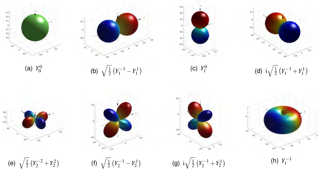
Figure 8.1: Polar plots (see §7.5 for details) of a few spherical harmonics Y_l^m(\theta, \phi) with l = 0, 1 or 2 . Notice that the familiar “orbital” shapes are often linear combinations of two Y_l^m(\theta, \phi) . Cases (a–g) are all real valued. Case (h) plots Y_1^{-1} which is complex valued. As explained in §7.5, the radius is determined by |Y_l^m| and the colouring by its real part.
