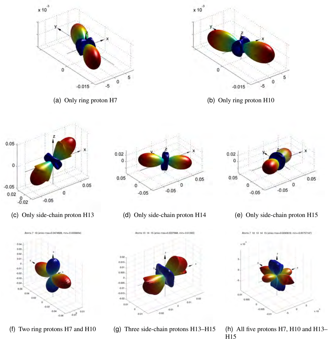
Figure 7.21: Polar plots of the singlet yield anisotropy in a series of “n=0” radical pairs containing a selection of magnetic nuclei from the Y^{\bullet} radical. The atom numbering and HFTs are shown in Figure 7.18. Calculations were made with an applied field B_0 = 50 \mu\text{T} and k = 2 \times 10^5 \text{ s}^{-1} , giving a radical pair lifetime of 5 \mu\text{s} .
