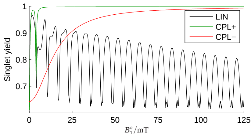
Figure 5.36: B_1 spectrum showing limiting behaviour in (unattainably) strong RF fields. RF field strengths for LIN polarised fields are described in terms of the strength of their CPL+ component B_1^0 = B_1/\sqrt{2} (see §5.2.4). Calculations were made using \gamma -COMPUTE or the RFT. Parameters: a = 0.5 mT, \nu_{\text{rf}} = 112 MHz, B_0 = 4 mT, k = 2.8 \times 10^7 s ^{-1} , n = 256 and \theta = \pi/2 . This figure has been checked for convergence by recalculating several points with n = 512 .
