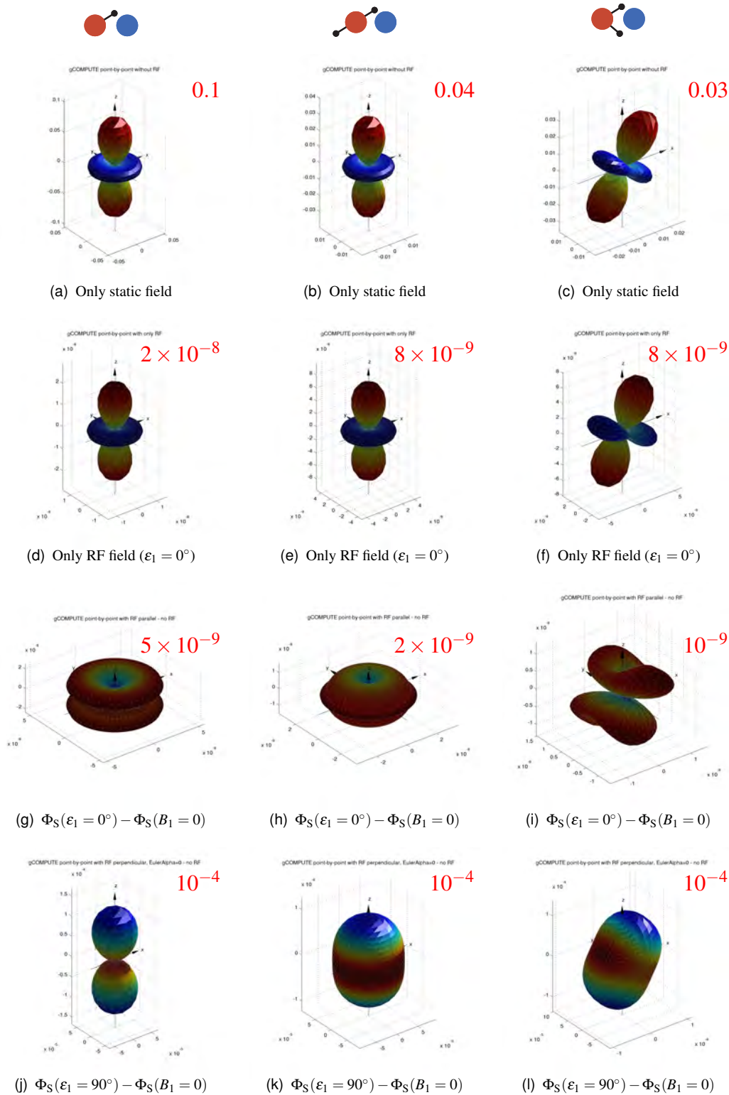
Figure 9.10: Effect of simultaneous static B_0 = 46 \mu\text{T} and RF B_1 = 33 \text{ nT} fields on the singlet yield of simple “1–0” and “2–0” model RPs. The maximum absolute value in each figure is shown in red. In all cases, the initial static field orientation \varepsilon_0 = 0^\circ , the rate constant k = 5 \times 10^4 \text{ s}^{-1} and the radio frequency \nu_{\text{rf}} = 1.3 \text{ MHz} . Hyperfine tensors with a = 500 \mu\text{T} , \alpha = -150 \mu\text{T} and \beta = 0 \mu\text{T} ; and a = 730 \mu\text{T} , \alpha = -153.3 \mu\text{T} and \beta = 0 \mu\text{T} were used. The cartoons at the top indicate how many HFTs were used and their relative orientation. In the right-hand column, the second HFT was rotated so that it was not coaxial with the first.
