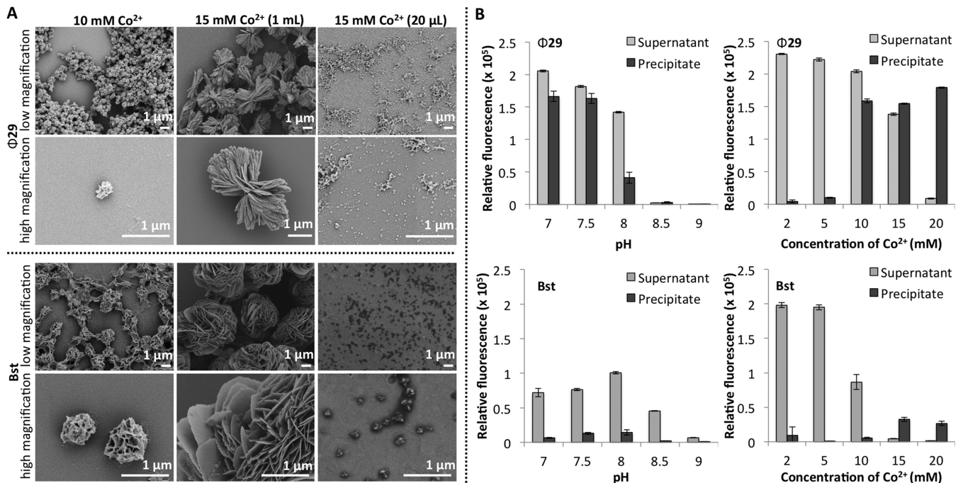
Figure 4. A) SEM images illustrating the effect of CoCl 2 concentration and reaction scale on the morphology and size of particles formed during RCA at pH 7.0. The Bst RCA incubation time was 14 h whereas the Φ29 incubation time was 20 h. B) Fluorescence-based analysis comparing the levels of free DNA and DNA incorporated into the nanoconstructs as a function of enzyme, pH, and cation concentration. Samples were broken down using TBE to release DNA prior to incubation with SYBR gold. A plate reader was then used to compare the DNA levels. The effect of pH on Φ29 and Bst RCA was determined at 10 mM CoCl 2 and the effect of concentration was evaluated at pH 7.0.
