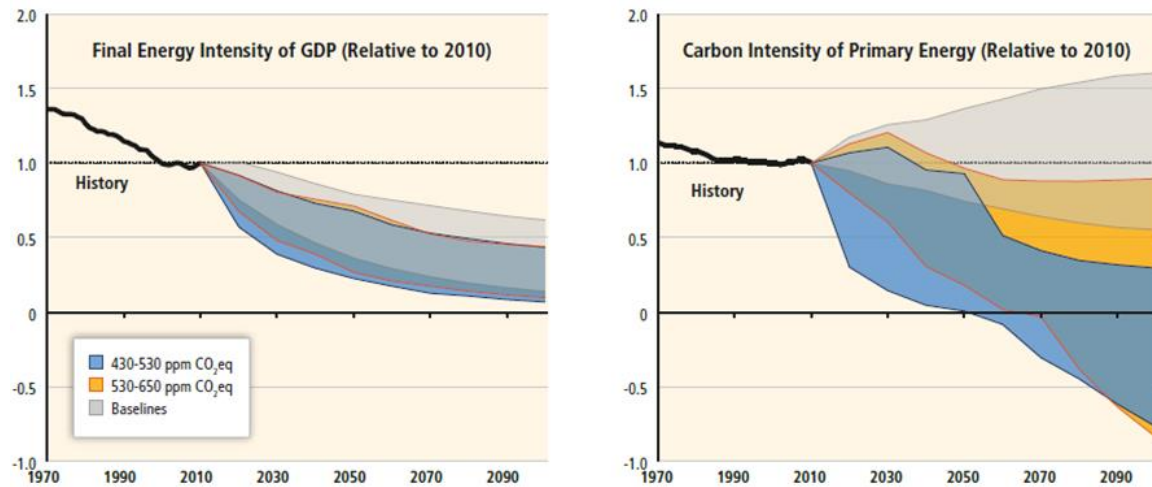
Figure 1. Contributions to global decarbonisation from energy and carbon intensity change for various carbon dioxide scenarios (IPCC, 2014)
