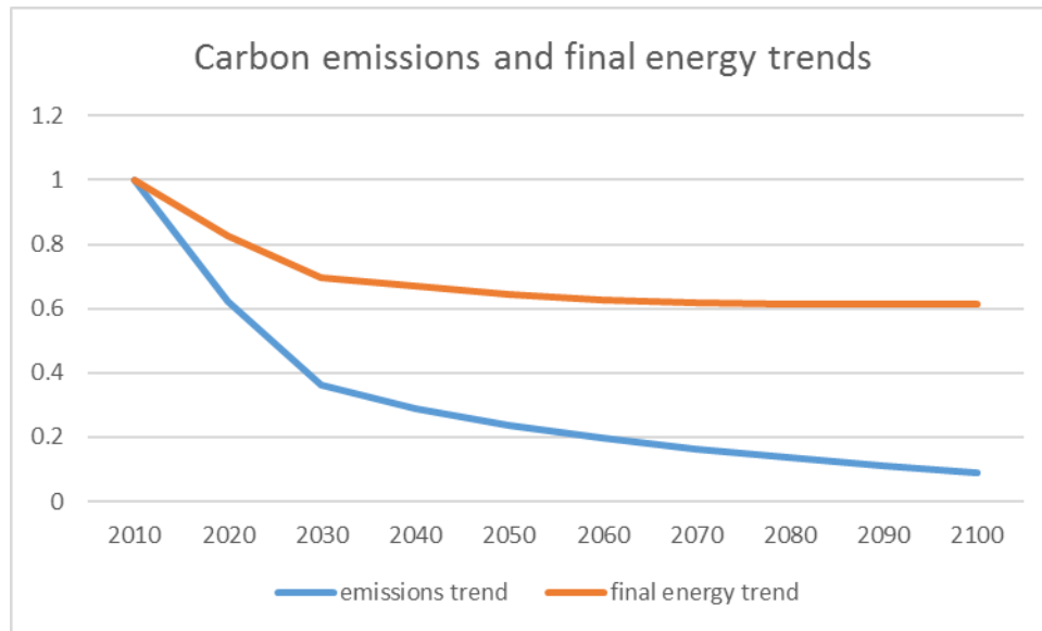
Figure 3. Example global model output of final energy and carbon emissions trends for an ambitious decarbonisation scenario. POLES model run for OECD, EMF 27 comparison exercise, EERE variant. Author calculations with data IPCC scenario data downloaded from http://www.iiasa.ac.at/web/home/research/researchPrograms/Energy/IPCC_AR5_Database.html
