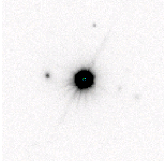
Figure 7. A 60 \times 60 arcsecond image from the SDSS DR7 r -band. The companion to the west is \sim 14 arcseconds away, and is 5.6 magnitudes fainter than EPIC 245950175 in R .
