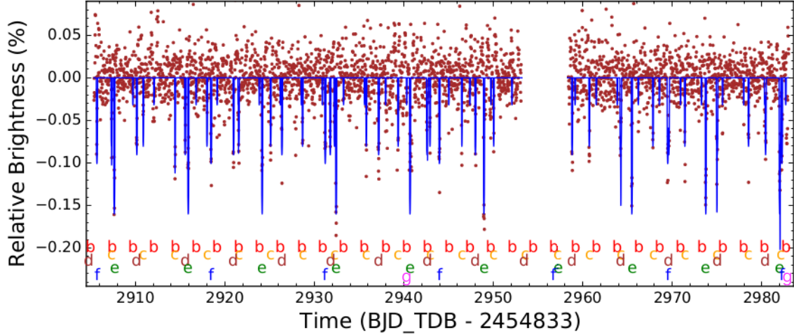
Figure 4. The time series of the K2 data, with the five-planet transit model shown in blue. The planets of the individual transits are marked with the appropriate letter; the times of the two transits of the putative planet candidate discussed in Section 3 are shown as ‘g’. The 5-day gap two-thirds of the way through the campaign was the result of a spacecraft safe-mode event.
