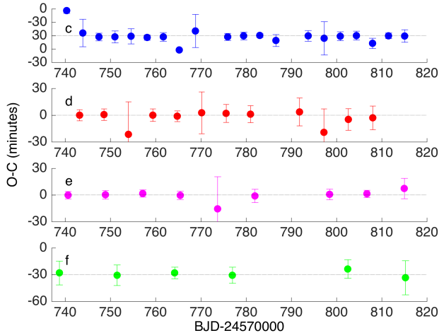
Figure 9. Examining the transit times of K2-138 c, d, e, and f. There are no significant variations observed at the timing precision of the K2 30-minute cadence observations.
