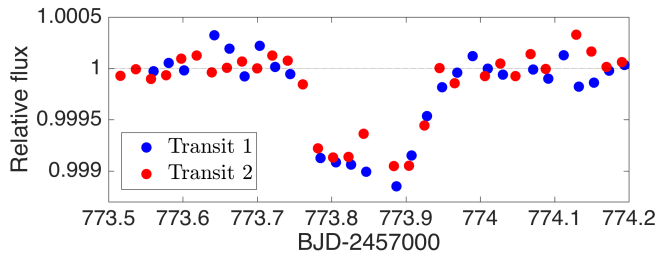
Figure 3. The two transits of the putative 42-day period planet candidate that fall in the K2 C12 data. The time of the second transit has been offset by 41.97 days to demonstrate the consistency in depth and duration of the two events, which correspond to a \sim 2.8R_{\oplus} planet.
