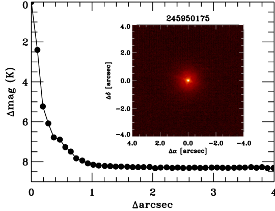
Figure 5. Inset: The Gemini/NIRI AO image of K2-138. We detect no additional sources of flux. Plot: The 5- \sigma contrast limits for additional companions, in \Delta magnitude, are plotted against angular separation in arcseconds; the black points represent one step in the FWHM resolution of the images.
