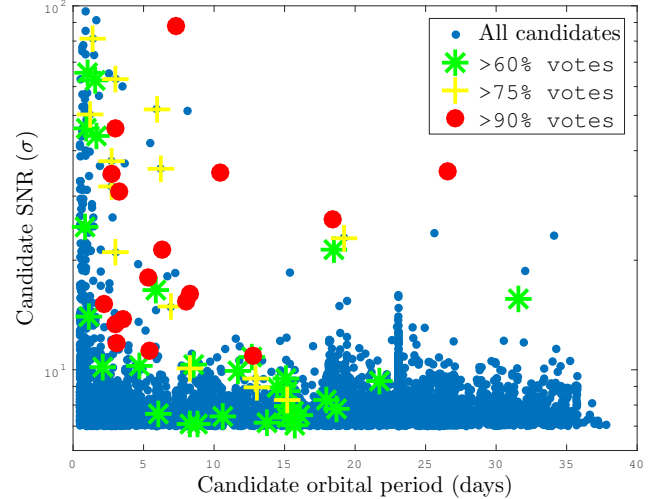
Figure 2. The distribution of user votes on the C12 candidate transiting planet signals. All signals received 14 or more votes, and the percentage of ‘yes’ votes is shown: the small blue dots represent signals for which fewer than 60% of users voted ‘yes’. The green stars, yellow + symbols and red circles show signals for which greater than 60%, 75% and 90% of users voted ‘yes’.
