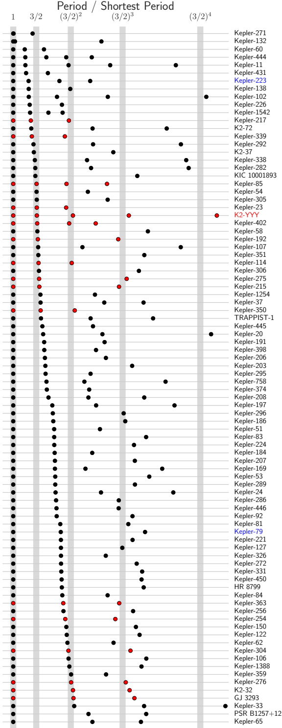
Figure 8. The distribution of distances from 3:2 period ratios in confirmed multi-planet systems that have three or more planets in a compact geometry (defined as having three planets with Period/Shortest Period < 4 ). Planetary systems with multiple near-3:2 resonances are highlighted in red. K2-138 is the only system near an unbroken chain of four near-3:2 resonances. Kepler-79 and Kepler-223 (shown in blue) both have four planets in or near a chain of resonances. The vertical lines indicate the positions of successive 3:2 period ratios.
