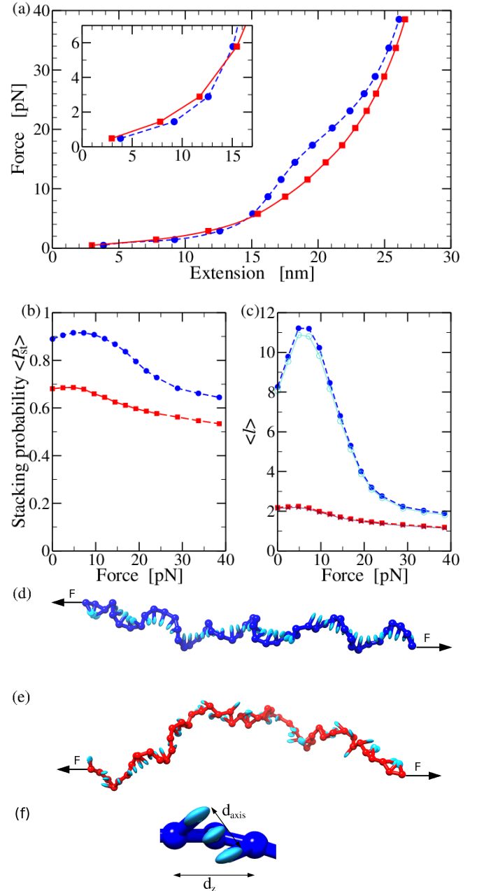
FIG. 7. (a) Extension of 50-nucleotide single-stranded DNA at 25 °C as a function of applied force. In all panels, blue circles correspond to a poly(dA) sequence (strongest stacking in our model), while red squares correspond to a poly(dGdA) sequence (weakest stacking). The inset in (a) shows a magnified section of the force-extension curve for low forces. (b) Stacking probability of a neighbor pair as a function of the applied force F . (c) Average length of a stacked domain \langle l \rangle as a function of applied force F . The open circles and crosses show \langle l \rangle_{\text{uncoop}} as predicted by the uncooperative stacking model (Eq. 11) using \langle P_{st} \rangle as measured for poly(dA) and poly(dGdA) respectively. (d) Visualization of a 50-base long poly(dA) ssDNA under a tension F = 15 pN, showing multiple stacked regions with helical geometry. The arrows indicate the applied force on the first and the last base. (e) Poly(dGdA) strand under a tension of 15 pN, consisting of short stacked regions as well as unstacked ones. (f) Magnified section of ssDNA illustrates that three stacked bases can align with the applied force without disrupting the stacking interaction. The contour length d_z , aligned with the force, is larger than the axial rise d_{\text{axis}} .
