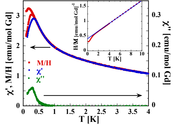
FIG. 2. Magnetization M/H (red points) and AC susceptibility vs T . \chi' (blue points) and \chi'' (green points) are the in phase and out of phase parts of the AC susceptibility. For the magnetization, the applied DC field is 5 mT. The AC susceptibility was measured in zero DC field with \mu_0 H_{AC} = 0.55 mT and f = 0.57 Hz. Inset: H/M \approx 1/\chi vs T for temperatures between 100 mK and 10 K. The blue line is a fit to a Curie-Weiss law between 20 and 300 K: 1/\chi = 0.499 + 0.128 T .
