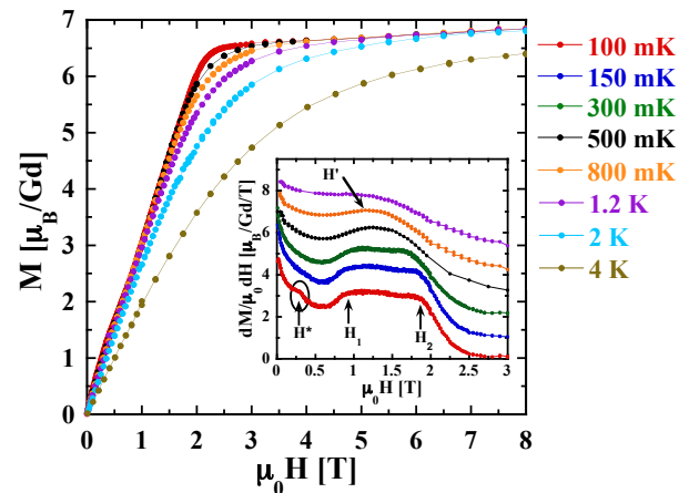
FIG. 3. M vs H for temperatures between 100 mK and 4 K. Inset: dM/dH vs H . The curves for different temperatures are shifted by steps of 1 \mu_B/\text{T} for clarity.
