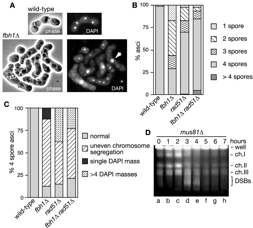
Figure 5. Meiotic chromosome segregation in a fbh1 Δ mutant. (A) Phase contrast and epifluorescence microscopy of DAPI-stained asci from wild-type (MCW1195 × MCW1196) and fbh1 Δ mutant (MCW1785 × MCW1832) homozygous crosses. The arrow indicates an example of where the DAPI-stained DNA in an ascus has failed to segregate and consequently is encapsulated in only one of the four spores. (B) Quantification of data like in (A) showing the percentage one-, two-, three- and four-spore asci obtained from wild type, fbh1 Δ, rad51 Δ (FO1033 × FO1541) and fbh1 Δ rad51 Δ (MCW1587 × FO1554) homozygous crosses. Values are based on the analysis of 150 asci from three independent crosses. (C) The percentage of four-spore asci obtained from wild-type and fbh1 Δ homozygous crosses that have uneven chromosome segregation between the spores. Values are based on the analysis of 100-four-spore asci from three independent crosses. (D) Pulsed field gel-electrophoresis analysis of chromosomal DNA from a mus81 Δ ( MCW2738 ) pat1-114 meiosis.
