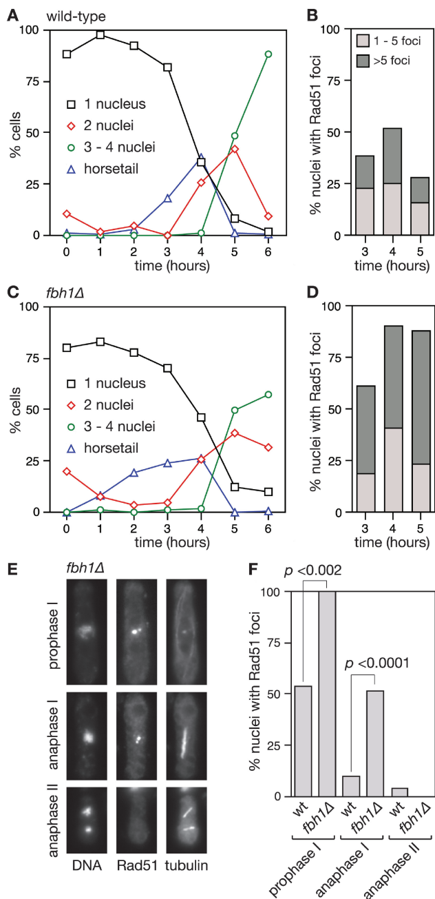
Figure 6. Rad51 foci accumulate to higher levels in a fbh1Δ mutant meiosis compared to wild type. (A) Cytological analysis of meiotic progression in a wild-type (MCW352) pat1-114 haploid meiosis. (B) Quantification of Rad51 foci in nuclear spreads obtained from the time course in (A). The spreads were stained with an antibody against Rad51. (C) Cytological analysis of meiotic progression in a fbh1Δ (MCW2138) pat1-114 haploid meiosis. (D) Quantification of Rad51 foci in nuclear spreads obtained from the time course in (C). The values in (B) and (D) are each from a single experiment in which 100-spread nuclei were analyzed for each time point. Experiments were repeated twice to confirm that the data were reproducible. (E) Representative images of fixed whole cells from a fbh1Δ mutant pat1-114 haploid meiotic time course stained for Hoechst 33342, Rad51 and tubulin. (F) Quantification of the number of fixed whole cells that stain positive for Rad51 foci at different stages of a pat1-114 haploid meiosis ( n = 30-40 ). P -values were determined using Fisher's Exact Test (two-tailed).
