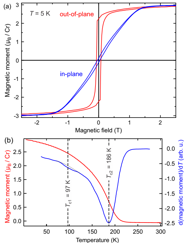
FIG. 1. (a) M(H) hysteresis loops for a \text{Cr}_{0.71}\text{Sb}_{1.29}\text{Te}_3 thin film sample with the field applied in-plane (blue) and out-of-plane (red). The data was taken at 5 K. (b) The temperature dependent magnetization, M(T) , was measured in an applied out-of-plane field of 20 mT during cool-down (red curve). The differentiated curve (shown in blue) reveals two transition temperatures.
