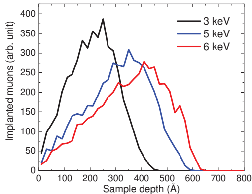
FIG. 8. Muon stopping profiles as a function of sample depth for the implantation energies used in this study. A depth of 0 Å denotes the sample surface.
