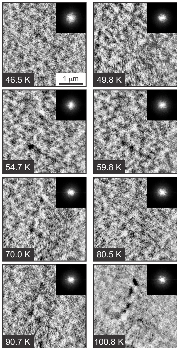
FIG. 4. XPEEM images, taken at the Cr L_3 edge at different temperatures ranging from 46.5 to 100.8 K. The scale bar ( 1 \mu\text{m} ) is shown in the top-left image, and is the same for all temperatures. In the top-right corner of each image, a Fourier transform of the contrast is shown. The XPEEM contrast has been normalized.
