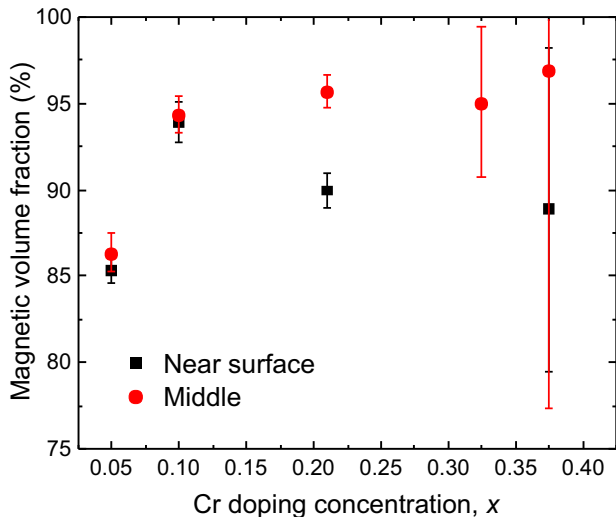
FIG. 7. Magnetic volume fraction as a function of Cr doping concentration at 4 K, both near the surface and in the middle of the films.
