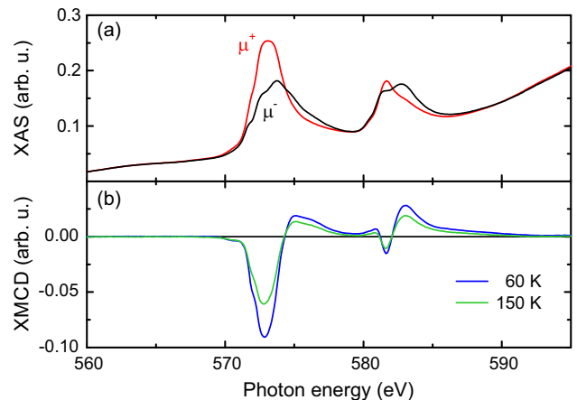
FIG. 2. Cr L_{2,3} spectra of Cr-doped Sb_2Te_3 ( x = 0.71 ) in an applied out-of-plane field of 2 T. (a) XAS spectra for opposite circular polarizations ( \mu^- , \mu^+ ) in normal incidence at 60 K. (b) XMCD ( \mu^- - \mu^+ ) spectra at 60 K (blue line) and 150 K (green line).
