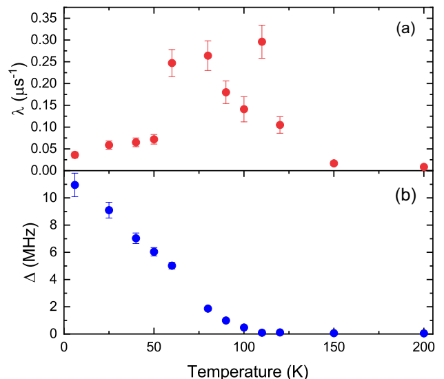
FIG. 6. Zero field measurement of the x = 0.325 sample at 6 keV, fit parameters vs temperature: (a) slow relaxation component \lambda , and (b) fast relaxation component \Delta .
