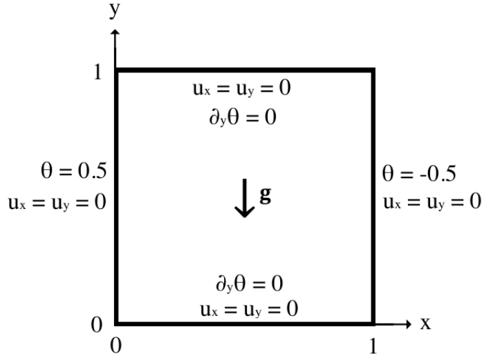
Figure 2: Geometry and boundary conditions for square cavity problem.
