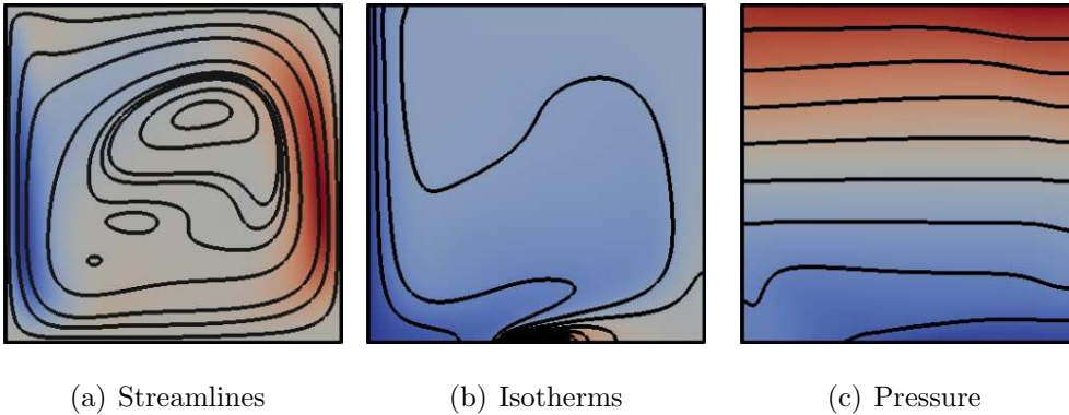
Figure 4: Contours of flow fields for convection in a partially heated cavity.
