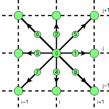
Figure 1: The D2Q9 lattice. The D2Q5 lattice does not have the diagonal links.
