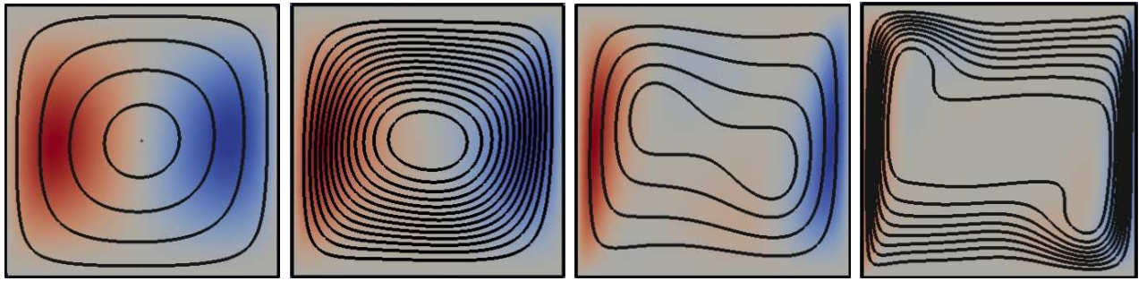
(a) Streamlines
