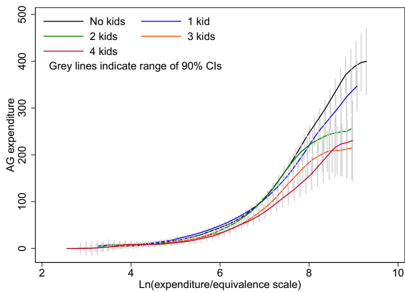
FIG. 3: LOCAL LINEAR REGRESSIONS OF ADULT GOOD EXPENDITURE ON COMPENSATED LN(EXPENDITURE): 2 ADULT HOUSEHOLDS, BY NO. OF CHILDREN
