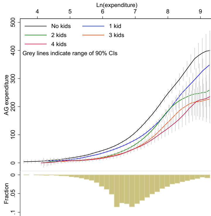
FIG. 2: LOCAL LINEAR REGRESSIONS OF ADULT GOOD EXPENDITURE ON LN(TOTAL EXPENDITURE): 2-ADULT HOUSEHOLDS, BY NO. OF CHILDREN
