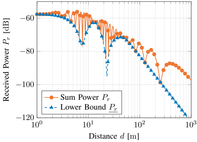
Fig. 6. Received power for two parallel frequencies with f_1 = 2.4 GHz, \Delta f = 250 MHz, h_{Tx} = 10 m, and h_{Rx} = 1.5 m. Both the actual value P_r from (11) and the lower bound \underline{P}_r from (12) are shown. (Example 4)
