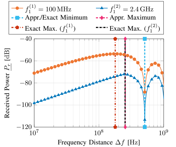
Fig. 7. Received power envelope \underline{P}_r for two parallel frequencies f_1 and f_2 = f_1 + \Delta f . The additional parameters are set to d = 50 m, h_{Tx} = 10 m, and h_{Rx} = 1.5 m. The first peaks are indicated, both the exact locations (numerically determined) and the approximations from Lemma 2. (Example 5)
