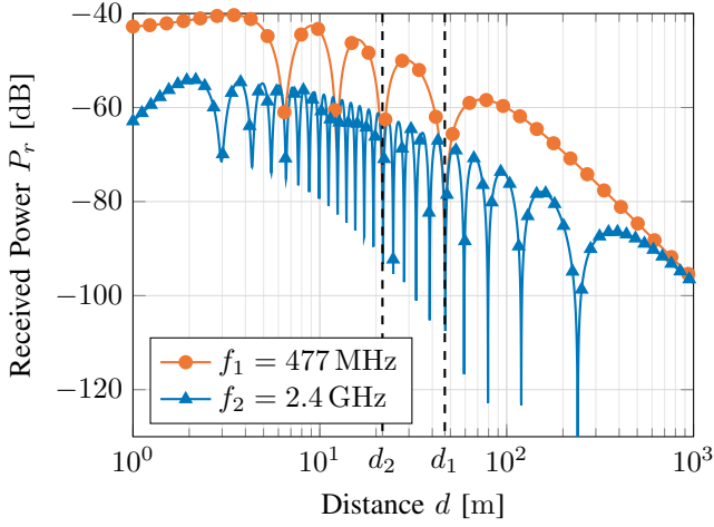
Fig. 4. Received power P_r(d) from (3) when using a single frequency f with system parameters h_{Tx} = 10 m, h_{Rx} = 1.5 m, \rho = 1 , \Gamma = -1 , and P_t = 1 for f = f_1 = 477 MHz and f = f_2 = 2.4 GHz. Additionally, the distances d_1(\omega_1) = 46.7 m and d_2(\omega_1) = 21.6 m from (9) are indicated. (Example 1 and Example 2)
