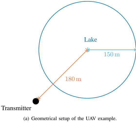
Fig. 12. Setup of the numerical example of a UAV flying above flat terrain. The movement of the UAV is modeled according to [37] with movement parameters \alpha_1 = \alpha_2 = 1 , \beta_1 = \beta_2 = 3 , \gamma_1 = \gamma_2 = 7 , \sigma_1 = \sigma_2 = 1 , and s_1 = s_2 = 1 . (Example 9)
