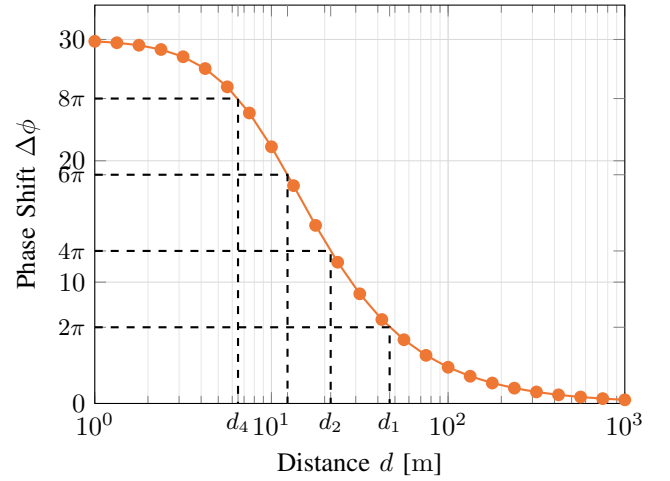
Fig. 3. Relative phase shift \Delta\phi from (8) for \omega/c = 10 , h_{\text{Tx}} = 10 m, and h_{\text{Rx}} = 1.5 m. Additionally the distances d_k , k = 1, \dots, 4 , from (9) are indicated. (Example 1)
