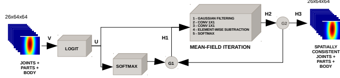
Figure 5: Spatial Model Architecture : the mean-field iteration module executes the mean-field update for T iterations. The additional modules pre-process the input unaries. Gates G1 and G2 switch outputs according to Eq. 6. References to the backward pass of the network are not included for simplicity.
