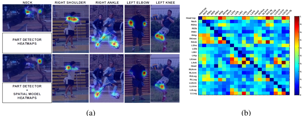
Figure 6: (a) Heatmaps from the LSP dataset. The first row shows heatmaps obtained from the part detector ( \mathbf{F}_1 ), while the second row shows heatmaps from the part detector plus the spatial model ( \mathbf{F}_1 + \mathbf{SM} ). (b) Learned Mean-field parameters: the higher the compatibility value, the higher the influence between the parts. We can notice small clusters of high influence, particularly between parts on the same side of the body (left/right), which explains how we mitigate double-counting.
