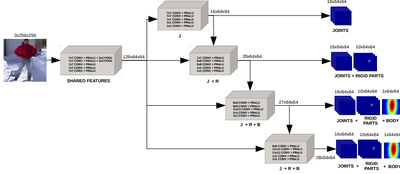
Figure 3: Multi-Level Body Part Detector Basic Architecture: a shared convolutional module produces CNN features that are used by subsequent modules to detect joints, rigid parts and the whole body. The initial detections of the joints (heatmaps) obtained by the module J – which can be seen as saliency maps (Itti et al., 1998) – are used to focus the visual attention (Borji and Itti, 2013) of the subsequent module J+R , which refines the previous predictions at the same time as it produces additional predictions for the rigid parts. The same principle is followed by the third module J+R+B , which refines the previous predictions and detects the whole body. The fourth module J+R+B is responsible for focusing on the person of interest, usually in the centre of the image. References to the backward pass of the network are not included for simplicity.
