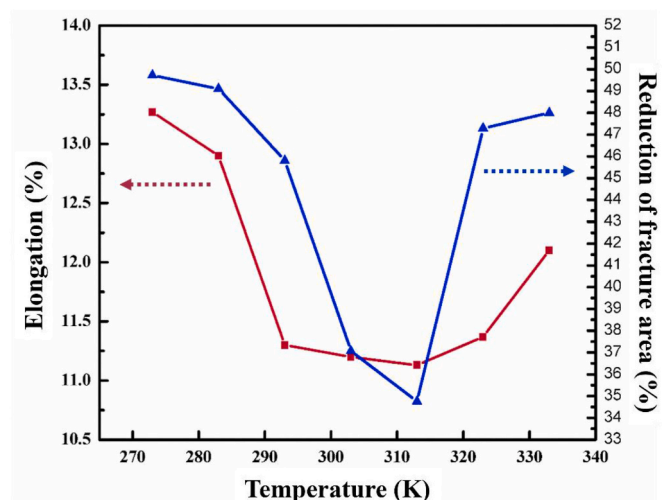
Fig. 6. Temperature window for HE. The extent of HE of hydrogen-charged ferritic/bainitic X90 pipeline steel specimens in terms of the reductions of elongation (red) and fracture area (blue). The HE reaches a maximum (300–320 K) close to room temperature (293 K). Properties were measured using slow strain rate tests with continuous hydrogen charging. Reproduced from [81] (For interpretation of the references to color in this figure legend, the reader is referred to the Web version of this article.)
