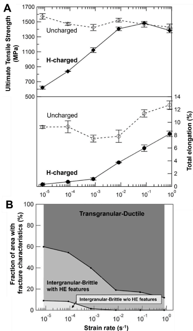
Fig. 7. The effect of strain rate on HE. (A) The UTS and the elongation of hydrogen-charged and uncharged low-carbon martensitic steel specimens decreased with decreasing strain rate in uniaxial tensile tests, showing HE is greater at lower strain rates. (B) Fractographic analysis of the specimens in (A) showing the surface area fraction of ductile and brittle features, indicating a change from transgranular-ductile to intergranular-brittle fracture with decreasing strain rate. Reproduced from [84].
