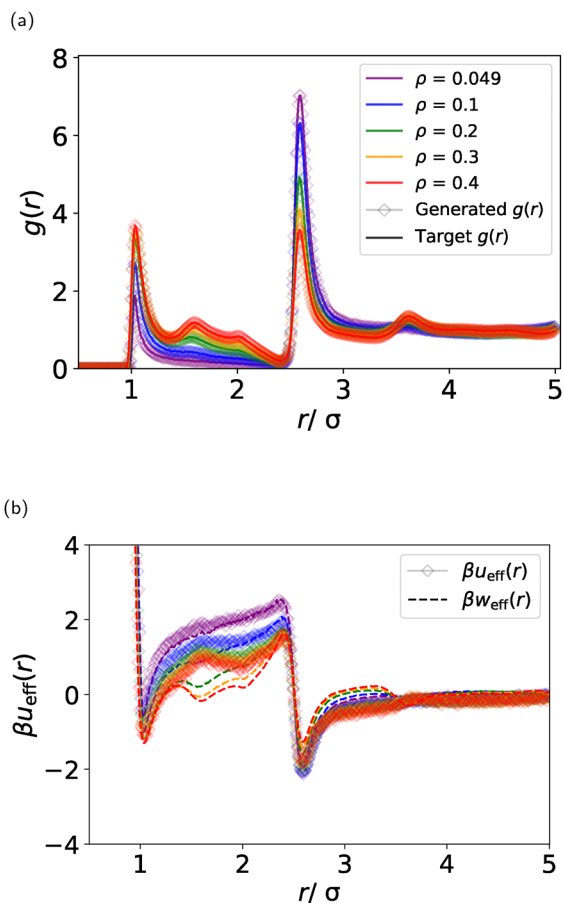
Fig. 5 Shoulder potential at varying density, with fixed Pe = 120 . (a) Plot comparing g_{\text{DH}}(r) and g_{\text{TP}}(r) , based on the converged \beta u_{\text{eff}}(r) from the inverse method. (b) Plot comparing \beta u_{\text{eff}}(r) with \beta w_{\text{eff}}(r) . The colour code in the key of (a) also applies to (b).
