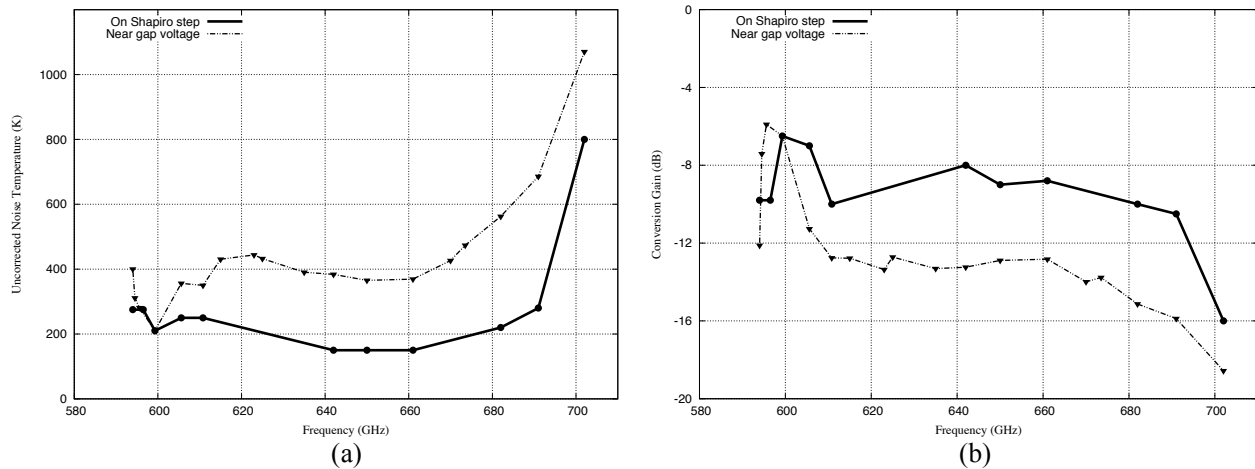
Fig.2 Multitude of the noise temperature improved by comparing the noise temperature measured at the first Shapiro step and the conventional bias point near the gap voltage. It is clearly seen that when the real first photon step is not available at higher frequencies end, the Shapiro steps measurement has a factor of \sim\sqrt{2} improvement.
