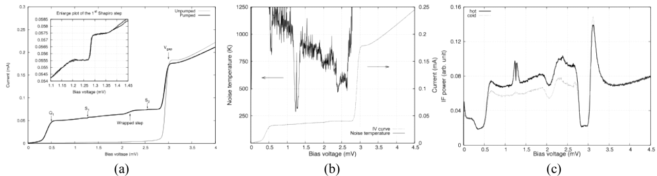
Fig.1 IV curve showing the step warping, the Shapiro steps and the photon steps at 634 GHz. Figure (b) plots the noise temperature calculated using the IF curves displayed in figure (c).
