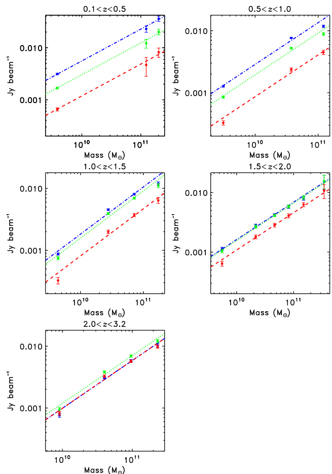
Figure A1. Stacked flux densities for the three different SPIRE bands, 250 μm (blue, dash-dotted), 350 μm (green, dotted) and 500 μm (red, dashed) plotted against the stellar mass of the galaxies for different redshifts. The dashed lines are the best fits of the model (equation 10). For every redshift and every SPIRE band, we can see a clear correlation of mass with flux density, so this plot is effectively another way to show the MS.
