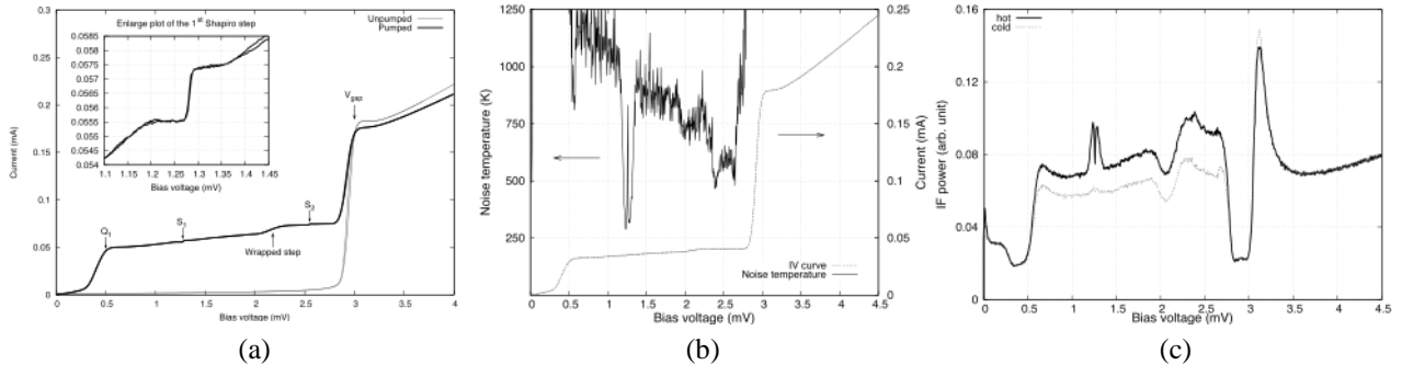
Fig. 1 IV curve showing the step warping, the Shapiro steps and the photon steps at 634 GHz. Figure (b) plots the noise temperature calculated using the IF curves displayed in figure (c).
