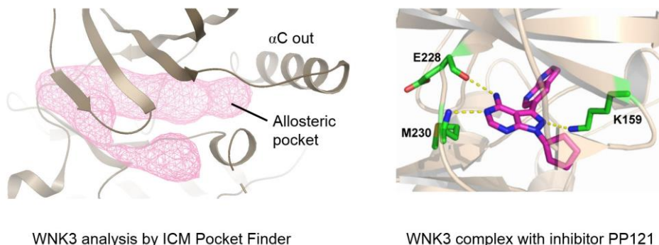
Fig. 8. PP121 inhibitor binding to WNK3
