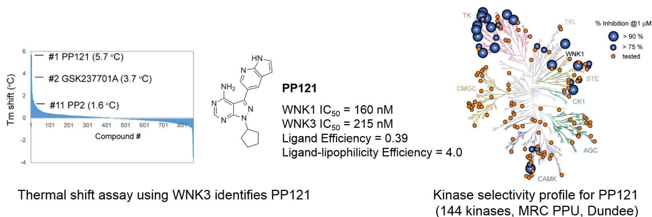
Fig. 11. Identification of PP121 as a WNK3 inhibitor
