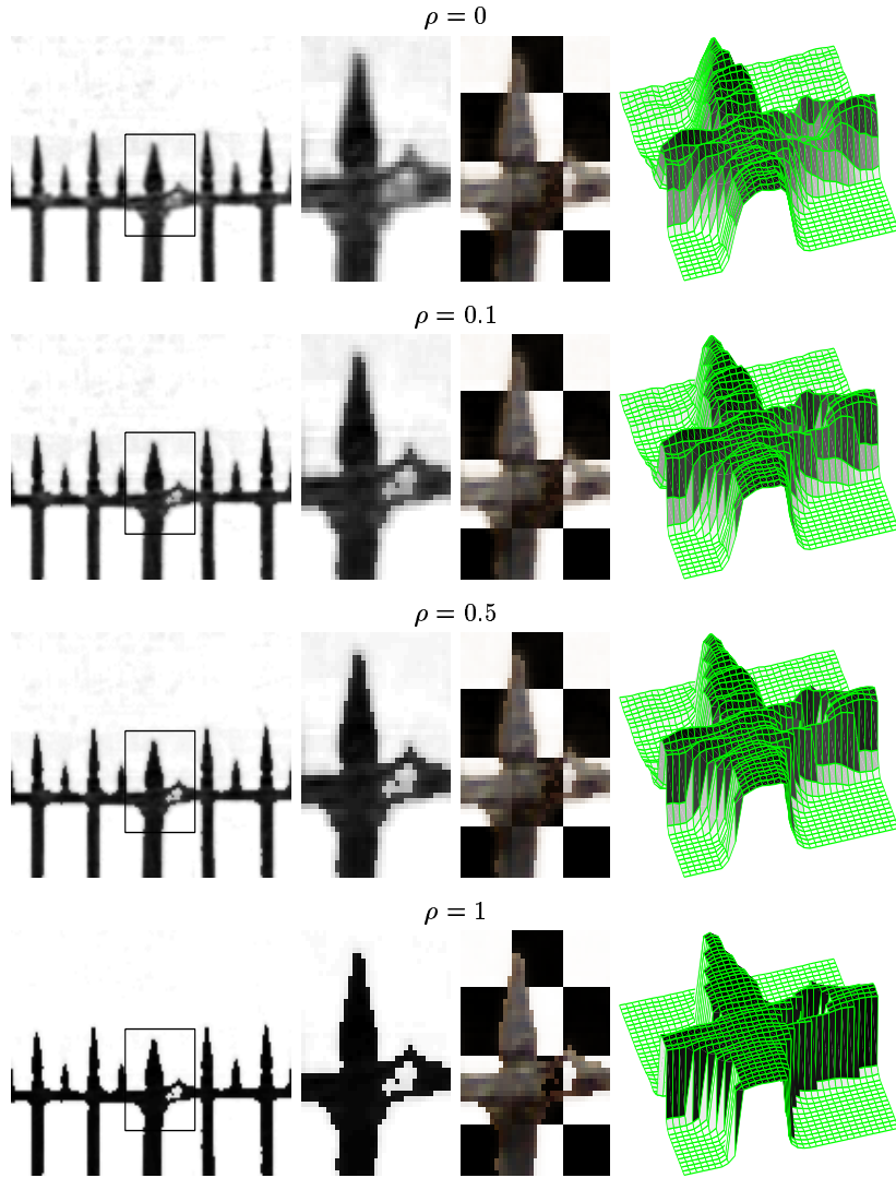
Fig. 5. Prior 2 , on the distribution of \alpha . As the prior on the distribution of \alpha increases, the mask becomes more binary. The figure is organized in columns: Left column shows the alpha mask where white colour marks transparent pixels and black marks opaque ones. Next is a zoomed portion of the mask on the left. The third column demonstrates the use of the mask for composition on a checkerboard pattern to emphasize both 'overshooting' and 'undershooting' of the values. The fourth column shows the alpha map as a height field. The reconstruction is shown for four values of the prior weight \rho . \rho = 0 is the MLE solution for which transparency is evident. As \rho increases, the matte is driven towards a binary image where pixels are labelled as purely foreground or background. Note that for \rho = 1 , the mask is binary and a halo is visible around the spearhead. This is evident in color images.
