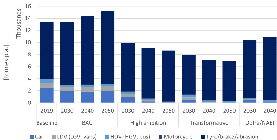
Fig. 8. Direct \text{PM}_{2.5} emissions from road transport, exhaust and non-exhaust. Notes: LDV = light duty vehicles (light goods vehicles, vans); HDV = heavy goods vehicles, trucks). Defra = Department for the Environment, Food and Rural Affairs. NAEI = National Atmospheric Emissions Inventory. Defra/NAEI data from Ref. [99].
