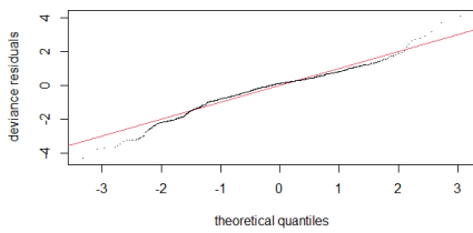
(a) Q-Q plot
