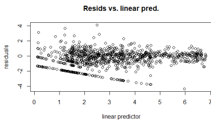
(c) Residuals versus Linear Predictor
