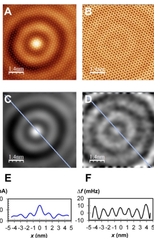
Figure 5. Central square (9 nm wide) within a 14 nm diameter quantum corral imaged at constant height by simultaneous STM (tunnelling current, left) and AFM (frequency shift, right). The data is recorded with a CO terminated tip, thus the atoms of the Cu(111) substrate appear as small maxima in A and as minima in B. C and D are low pass filtered versions of A and B, revealing the electronic states of the quantum corral. The STM data shows only the contribution of the electrons at the Fermi level, shown in blue in E. The AFM data shows the total charge density as plotted in F. From [63]. Reprinted with permission from AAAS.
