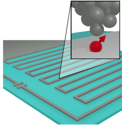
Figure 11. Atomic-scale STM experiments within a controlled electromagnetic environment as provided by carefully designed on-chip resonators may pave the way for new technological advances.
