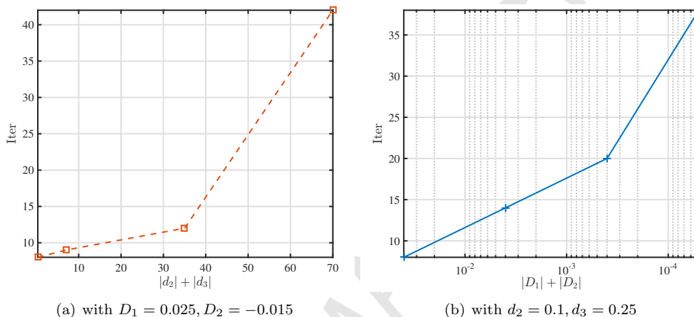
Fig. 5.5: Example 3: Iteration count produced when varying the coupling parameters defining the concentration-dependent body load and displacement-dependent source (a), and the stress-assisted diffusivity parameters (b).
