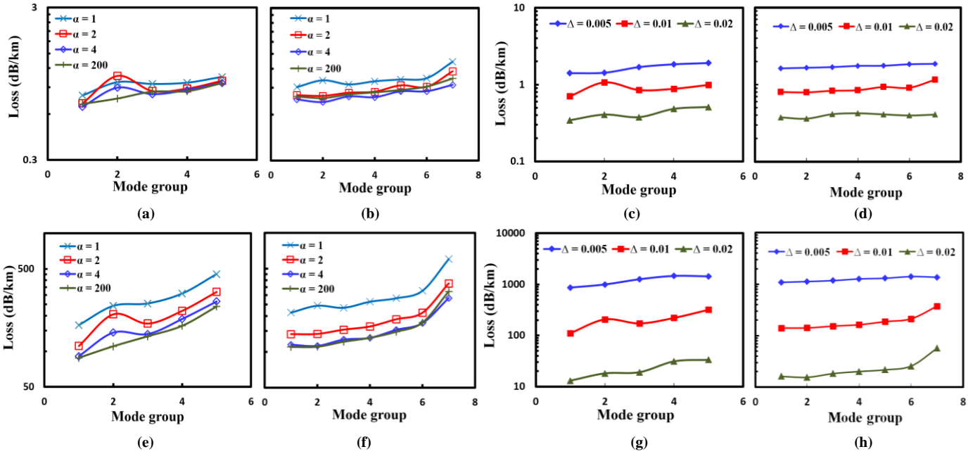
Fig. 6. Microbending loss of the 5/7-MG RCFs for different values of (a,b,e,f) \alpha ( \Delta=0.01 ) or (c, d, g, h) \Delta ( \alpha=2 ). \sigma=35nm (a-d): L_c=1mm , p=2 ; (e-h): L_c=0.083mm , p=3 .
