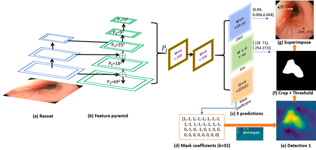
Fig. 4. The architecture of prediction head. (a) Backbone model Resnet. (b) Feature pyramid to extract features at each layer where P_3 = 69^2 , P_4 = 35^2 , P_5 = 18^2 , P_6 = 9^2 , P_7 = 5^2 . (c) The network outputs 3 predictions, class, box corner and 32 masque coefficients for each proposed anchor (A).
