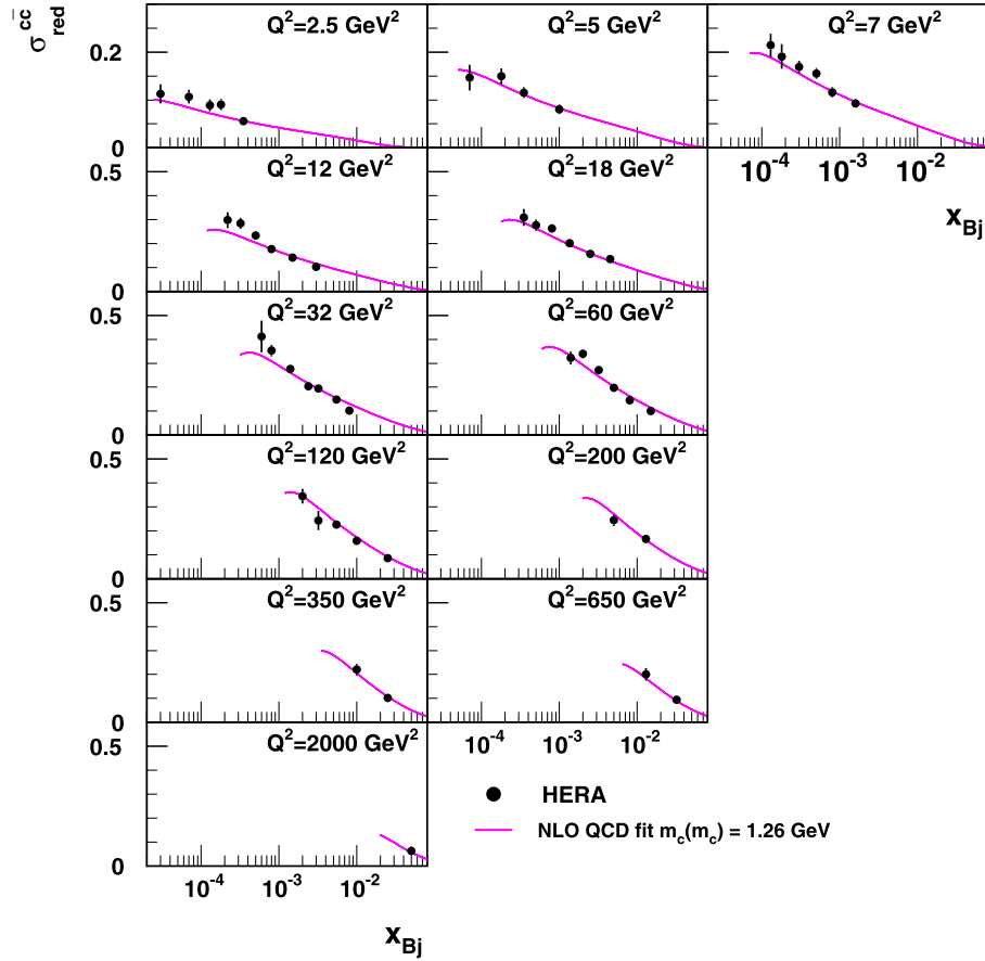
Fig. 1. Reduced cross section for charm production in deep-inelastic scattering [14] as a function of the Bjorken scaling variable x_{\text{Bj}} for different values of photon virtuality Q^2 (points). The measurements are grouped into six subsets in Q^2 , as indicated by the six rows, and detailed in Table 1. The curve shows the global NLO QCD fit for m_c(m_c) = 1.26 GeV described in the text.
