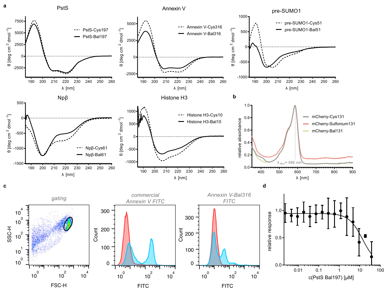
Extended Data Fig. 3 | Retention of fold and function after borylation. Retention of fold and function after borylation: (a) CD spectra of borylated proteins PstS-Bal197, Annexin V-Bal316, Npβ-Bal61, preSUMO1-Bal51 and Histone H3-Bal10 in comparison with their respective cysteine mutants. (b) Absorbance spectra of mCherry-C131, mCherry-Sulfonium131 and mCherry-Bal131 show unaltered absorbance maxima at 586 nm. (c) Annexin V-Bal316 binding to apoptotic cells (apoptosis induced using etoposide (ETO) at 25 \mu M concentration). (d) Inhibitor vs. response plot for competition of PstS-Bal197 with phosphate sensor. A stock solution of the commercially available, coumarin-dye labelled PstS variant 27 'Phosphate Sensor' (ThermoFisher Scientific, USA) and sodium phosphate in TRIS buffer (20 mM, pH 7.6) was prepared and titrated against PstS-Bal197, while the response was measured via fluorescence readout. Values represent mean \pm SD. n = 3 .
