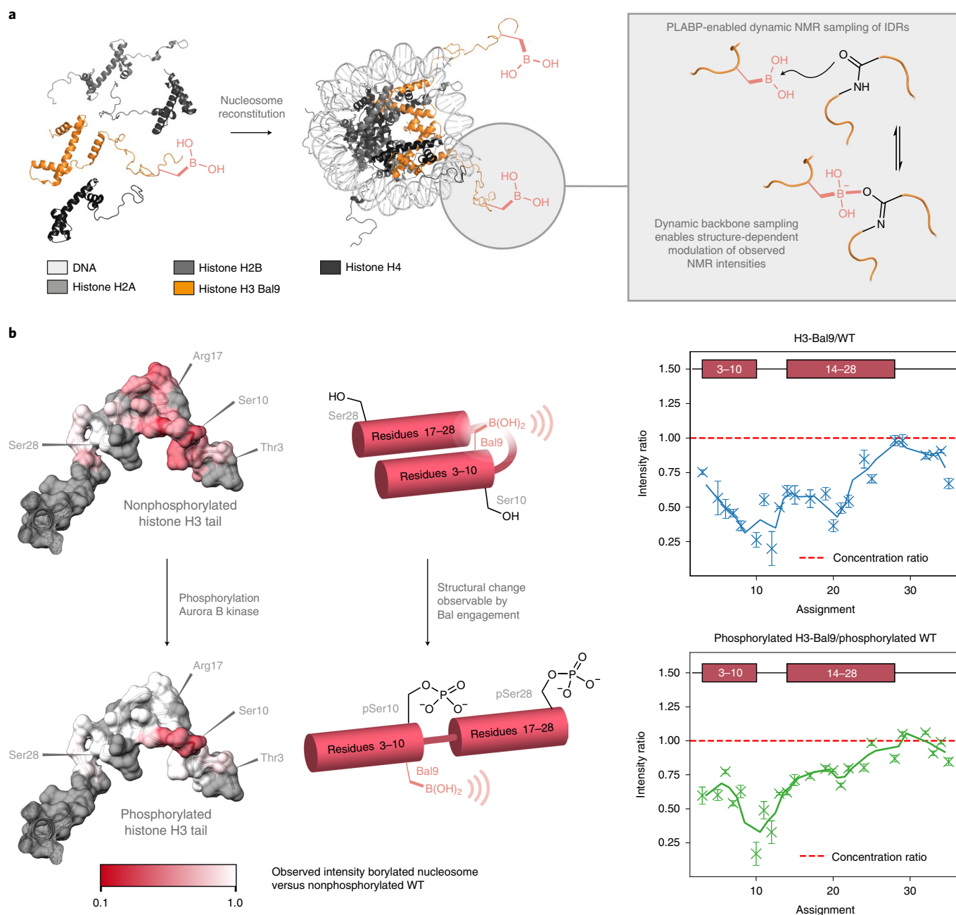
Fig. 6 | Exploitation of Bal in PLABP using the DICE method as a direct probe of IDRs found during epigenetic modification in nucleosomes. a, Assembly of nucleosomes containing histone H3-Bal9 allowed for exploitation of dynamic PLABP for the probing of structure via NMR using DICE. b, Nucleosome phosphorylation leads to a structural change in the tail of histone H3 that can be observed as a change in Bal-mediated backbone binding. Bal acts as a direct NMR ‘observer’ sensitive to structural change. Comparison of the NMR intensities of borylated and WT nucleosomes uniquely reveals both short- and long-range structural information. Comparison of intensity modulation after phosphorylation of both Bal-containing nucleosomes and WT nucleosomes reveals no notable differences, confirming Bal’s benign nature as an ‘observer’. Values represent the mean \pm s.d. from n=3 measurements of the same sample.
