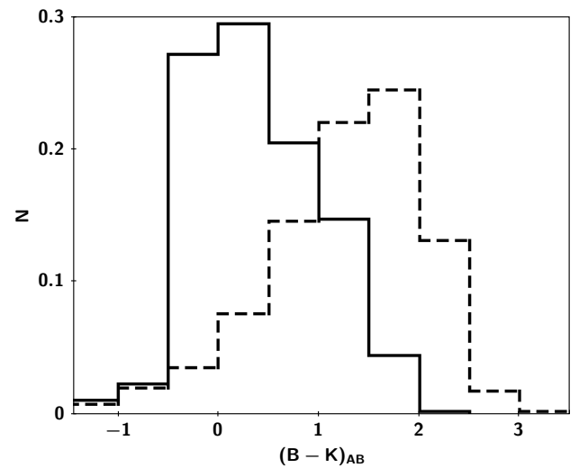
Fig. 6. The distribution of the B-K colour for galaxies in the Local Universe (dashed line) monitored by the LOSS survey (Li et al. 2011), and for galaxies in the SUDARE sample (solid line). We converted colours in Li et al. (2011) from the Vega to the AB magnitude system.
