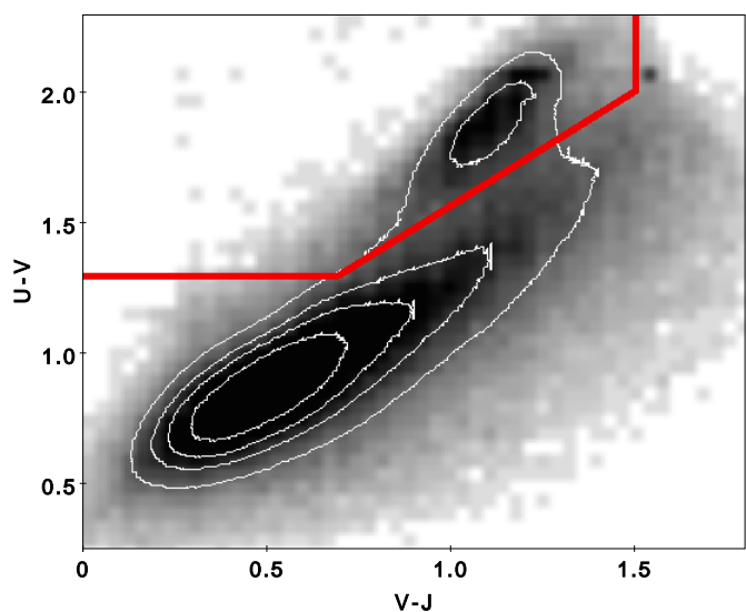
Fig. 3. The rest frame U - V vs V - J colour-colour diagram for the CDFS galaxy sample. The solid red line separates passive from star-forming galaxies (Eq. 1).
