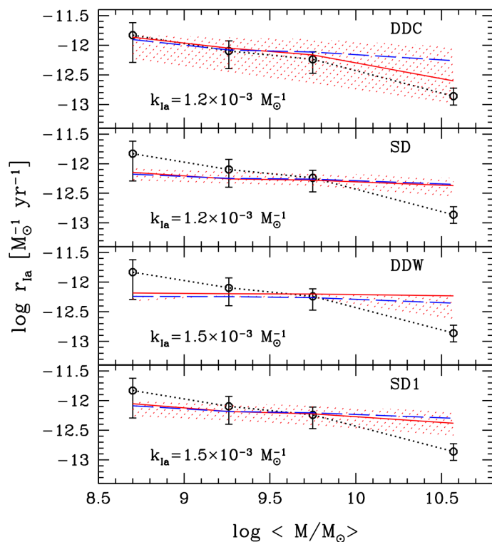
Fig. 16. SN Ia rate as a function of galaxy mass. Black circles are the observed rates in the four mass bins, reported in Table 2, while lines connect the theoretical rates at the median \langle Age \rangle of the distributions in the four mass bins. Solid (red) and dashed (blue) lines refer to exponentially declining SFH models with \tau = 0.1 and 8 Gyr, respectively. The shaded areas show the range covered when using the 30-th or 70-th percentiles of the \langle Age \rangle distribution instead of the median \langle Age \rangle , for the exponentially declining SFH models with \tau = 0.1 Gyr.
