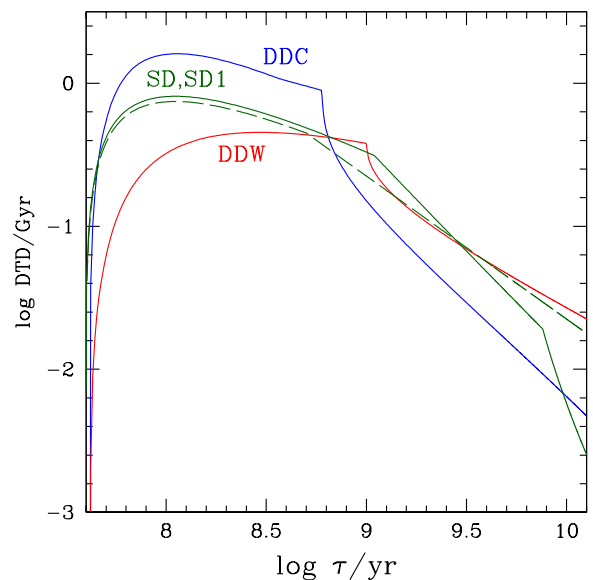
Fig. 11. Distributions of the delay times adopted in our modeling, selected from the family in Greggio (2005). SD (green solid): a single degenerate model which assumes Chandrasekhar mass explosions; SD1 (green dashed): the same as SD up to a delay time of 0.5 Gyr, proportional to the inverse of the delay time onward; DDC (blue): a DD CLOSE model with parameters \beta_a = -0.9 , \tau_{n,x} = 0.6 ; DDW (red): a DD WIDE model with parameters \beta_a = 0 , \tau_{n,x} = 1 . See Greggio (2005) for a description of the models. The DTD models are normalized to 1 over the range of delay times from 0 to 13 Gyr.
