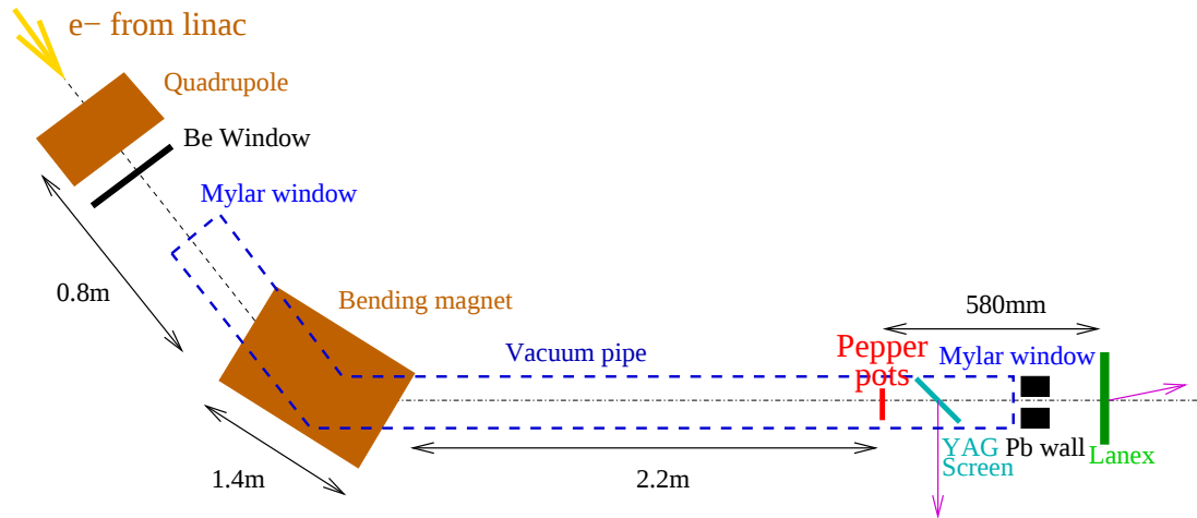
Figure 2: Experimental layout at the DAFNE BTF.
