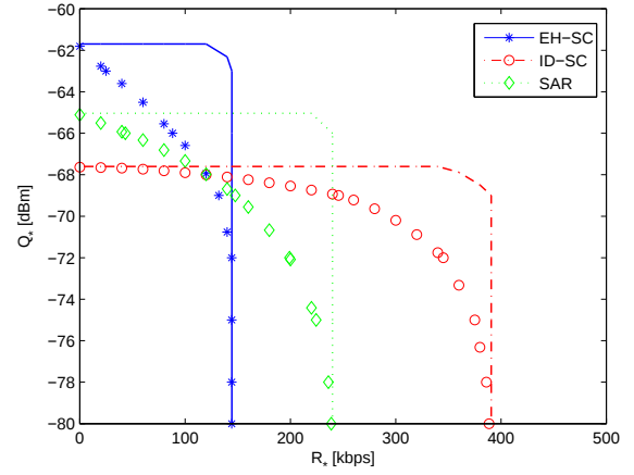
Fig. 2: Contour lines of the J-CCDF of SAR, ID-SC and EH-SC schemes. The curves show the pairs (R_*, Q_*) so that \bar{F}(R_*, Q_*) = 0.75 . Markers: Monte Carlo simulations. Solid, dotted and dashed lines: Proposition 2 .
