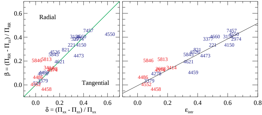
Figure 2. Left panel: the mass-weighted anisotropy parameter \beta \equiv 1 - \sigma_z^2/\sigma_R^2 versus the anisotropy \delta \equiv 1 - 2\sigma_z^2/(\sigma_R^2 + \sigma_\phi^2) measured from the orbital distribution of the 25 dynamical models, within the volume sampled by the observed kinematics. All objects, with the exception of the dwarf elliptical M32 (NGC 221), are early-type galaxies from the SAURON representative sample, and are also shown in the diagram of Fig. 3. The green line indicate galaxies with \sigma_R = \sigma_\phi . Most of the galaxies fall close to the green line, indicating that the anisotropy is characterized by a flattening of the velocity ellipsoid in the meridional plane, while the velocity ellipsoid tends to be circular in a plane parallel to the equatorial plane. The red and blue labels refer to the slow-rotators and fast-rotators respectively (see Fig. 1 for an illustration). Right panel: correlation between the intrinsic flattening \varepsilon_{intr} and the anisotropy parameter \beta . The flatter galaxies tend to be more anisotropic, as one may expect if the increasing flattening is due to a disk heating process.
