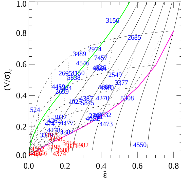
Figure 3. (V/\sigma) - \varepsilon diagram for all the 48 E/S0 galaxies in the SAURON representative sample (half of these objects are in common with Fig. 2). The kinematics were measured in a robust way from our luminosity-weighted integral-field kinematics (inside one R_e ) as (V/\sigma)_e^2 \equiv \langle V^2 \rangle / \langle \sigma^2 \rangle , following Binney (2005). The ellipticity \bar{\varepsilon} is luminosity-weighted within the same region adopted for the kinematics. The red and blue labels refer to the slow-rotators and fast-rotators respectively (see Fig. 1). The green line shows the location of oblate isotropic ( \delta = 0 ) edge-on galaxies, while subsequent black solid lines indicate increasing anisotropy values \delta = 0.1, 0.2, \dots, 0.6 . The magenta line corresponds to a linear relation between anisotropy \delta and ellipticity \varepsilon for edge-on galaxies. The dotted lines show the location of galaxies, originally on the magenta line, when the inclination is decreased i = 80^\circ, 70^\circ, \dots, 10^\circ . The dashed lines correspond to constant intrinsic ellipticity in the range \varepsilon_{\text{intr}} = 0.8, 0.7, \dots, 0.1 . While the fast-rotators can be described as a family of oblate anisotropic galaxies, seen at different inclinations, the slow-rotators are inconsistent with this distribution. The presence of kinematical misalignments indicates that the slow-rotators are (weakly) triaxial systems. The two galaxies NGC 4473 and NGC 4550 fall below the magenta line due to the strong tangential anisotropy (left panel of Fig. 2) caused by major counterrotating stellar disks (Rix et al. 1992; Cappellari & McDermid 2005).
