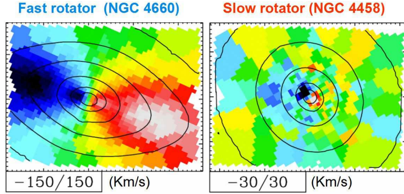
Figure 1. Mean stellar velocity field ( 30 \times 40 arcsec) observed with SAURON (from Emsellem et al. 2004) for two prototypical galaxies in the fast-rotators and slow-rotators classes respectively.
