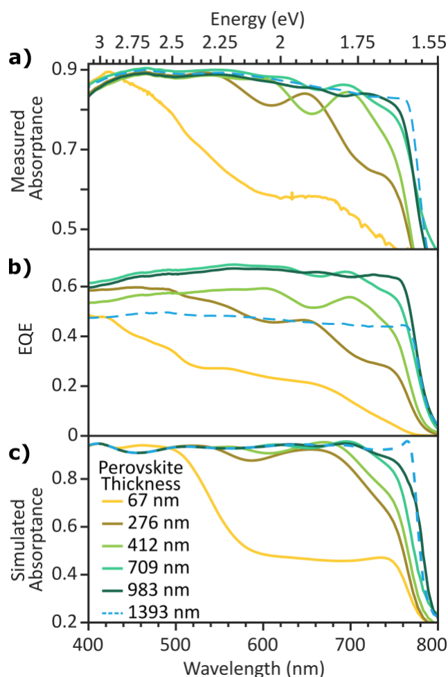
Figure 2. a) The measured absorption spectra of the devices shown in Figure 1 b) The external quantum efficiency (EQE) of the devices shown in Figure 1 c) The simulated absorption spectra for full devices (as shown in Figure 1) incorporating different thickness of perovskite thin films. The absorption spectra were simulated using a transfer matrix model created by Burkhard et al. [34] Detailed information of the model used can be found in the SI.
