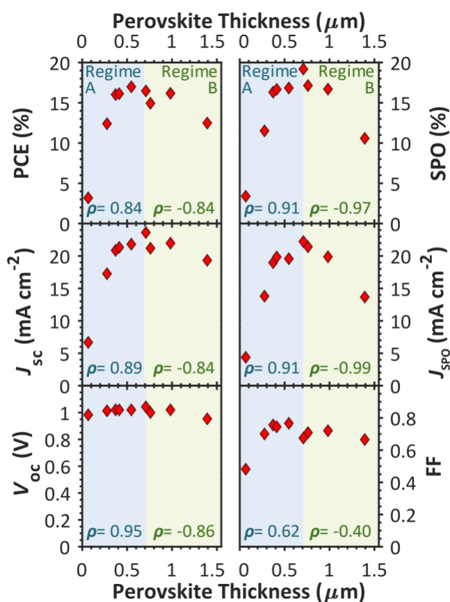
Figure 5. The device characteristics of vapor-deposited perovskite devices with different thicknesses of CH 3 NH 3 PbI 3 . The plots show the power conversion efficiency (PCE), the steady-state power output (SPO) at constant applied bias, the short circuit current density ( J_{sc} ) the steady-state current density ( J_{sp0} ) at constant applied bias, the open circuit voltage ( V_{oc} ) and the fill factor (FF). The red markers represent parameters obtained from J - V characterisation of the devices with the highest SPO at each thickness. The blue shaded region signifies devices which incorporates perovskite thin films \leq 709 nm and is termed ‘Regime A’. The green shaded region
