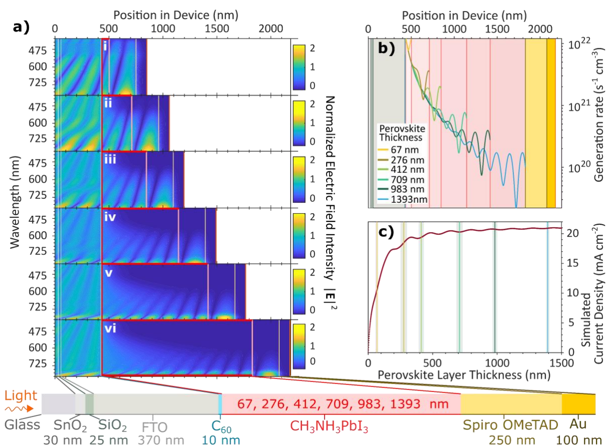
Figure 3 a) Simulation of the optical electric field within photovoltaic devices incorporating different thickness of perovskite thin films. The simulations show devices which incorporate i) 67 nm ii) 276 nm iii) 412 nm iv) 709 nm v) 983 nm vi) 1393 nm perovskite thin film thicknesses. The schematic at the bottom shows the direction of the incident light and the arrangement of layers and their thickness in the simulated device. b) Shows the generation rate of different thicknesses of perovskite thin films at different positions in the device. c) Shows the calculated
