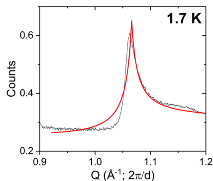
Figure 6. Fit to the peak at Q \sim 1.07 \text{ \AA}^{-1} when a Warren-like peak-shape function is used. The data is from the measurement of parent \text{Sr}_2\text{MnO}_2\text{Cu}_{1.82(2)}\text{Te}_2 at 1.7 K using the 2/9 bank of WISH ( 2\theta = 58.3^\circ ).
