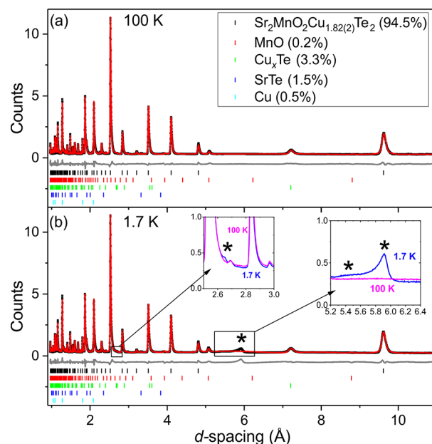
Figure 5. Rietveld fit to the WISH 2/9 bank ( 2\theta = 58.3^\circ ) data of \text{Sr}_2\text{MnO}_2\text{Cu}_{1.82(2)}\text{Te}_2 at (a) 100 K and (b) 1.7 K. The * symbols emphasize the peaks that appear on cooling and cannot be indexed using the nuclear model.
