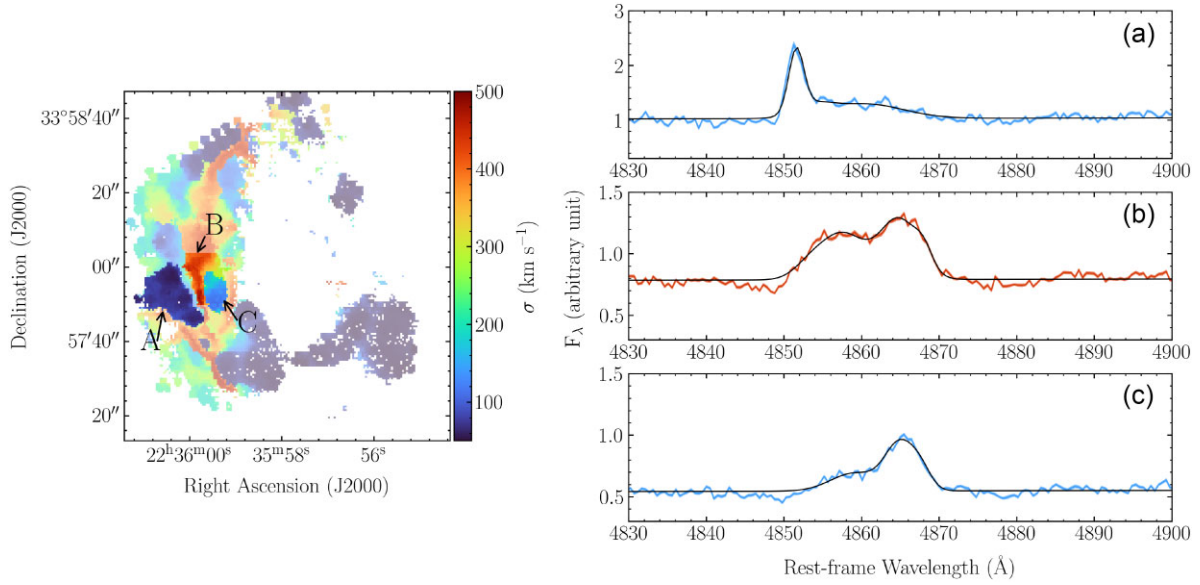
Figure A3. Line profiles in different regions of the LSSR around SQ. The left panel shows the velocity dispersion of H\alpha as in Fig. 3, along with three regions of interest as indicated by the arrows. The right panel presents the stacked spectra of these regions around the H\beta line (chosen since it is well isolated from other species, unlike e.g. H\alpha ), where the shaded area indicates the \pm 1\sigma uncertainty on the stack. The black solid line shows the best fit to the data, where the emission lines in all three stacked spectra has been modelled by four Gaussian components, as determined by the BIC.
