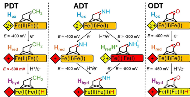
Fig. 3 Simplified representations of the H-cluster showing proposed pathways of H_{hyd} generation (see Fig. S6 for a more detail, ESI † ). [4Fe-4S]_H is shown as a diamond, [2Fe]_H as a rectangle, the dithiolate ligand as sticks and the CO/CN are omitted. The native, ADT-containing enzyme in H_{ox} is doubly reduced (on [4Fe-4S]_H and [2Fe]_H ) and protonated at the ADT bridgehead yielding H_{hyd} via H_{red} or H_{red}H^+ intermediates. Both reduction steps happen with redox potentials close to -400\text{ mV} . For PDT and ODT, reduction of [4Fe-4S]_H happens close to -400\text{ mV} (the dithiolate ligand has only a minor influence on the [4Fe-4S]_H redox potential). Reduction of [2Fe]_H in both the PDT and ODT cases proceeds without protonation of the dithiolate bridgehead, and the redox potential will depend on the stability of H_{hyd} . Electron withdrawal from the bridgehead group (O in ODT and CH_2 in PDT) is predicted to influence the electron density on the Fe ions with O more electron withdrawing than C. Hence, reduction of [2Fe]_H and H_{hyd} formation occurs at less negative potentials in the ODT enzyme than in the PDT enzyme.
