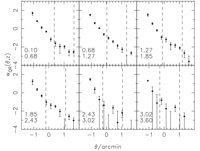
Figure 4. The quasar–radio source angular correlation function of our sample. The vertical lines are at 2 and 20 Mpc projected distance. The redshift limits for each bin are given in the bottom left of the panels.
