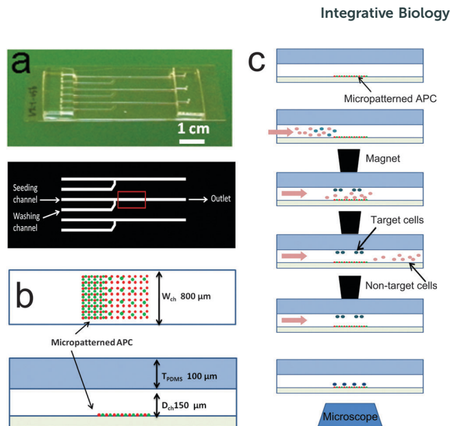
Fig. 1 A magnetic microfluidic chamber for improved cell microscopy. (a) Device design. (b) Schematics of top and side views of the red boxed area in (a). (c) Capture and isolation of paramagnetic beads-labeled cells are carried out using a diverging magnetic field, applied during cell loading. In this implementation, the magnetic field is applied using a stack of permanent magnets. When collection is finished, the magnet is removed and cells are released onto antibody patterns of interest (shown in red box in panel a and b).
